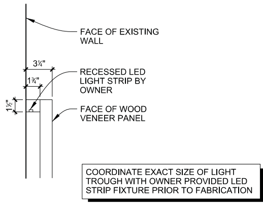
DETAIL E - TOP OF PANEL
