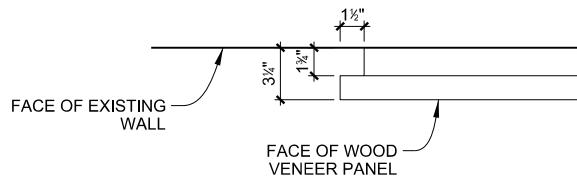
DETAIL F - SIDE OF PANEL
