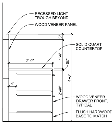
DETAIL C - TOP OF PANEL
