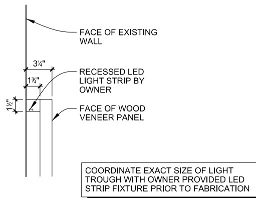
DETAIL B - TOP OF PANEL
