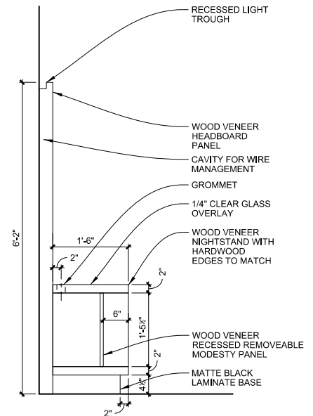
SECTION B - NIGHTSTAND
