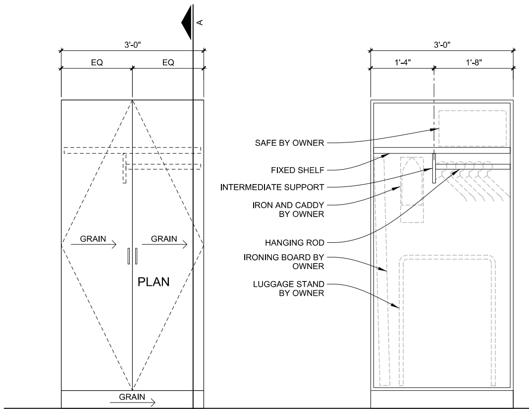
FRONT ELEVATION
