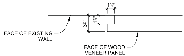
DETAIL C - SIDE OF PANEL
