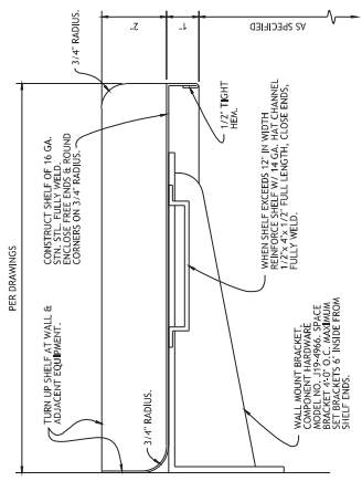
2 SECTION - ELEVATED SHELF NO SCALE REF: ITEM NO. 106, 126, 203, 205, 245, 247, 253 & 261
