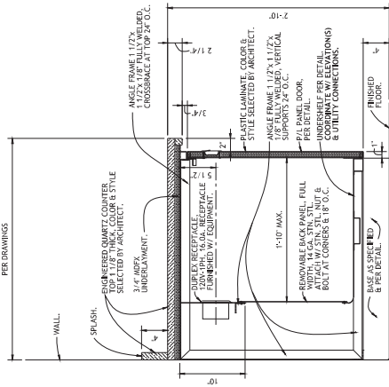
3 SECTION - BEVERAGE COUNTER
