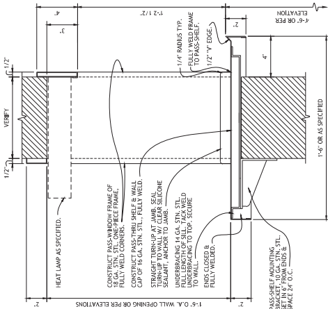
2 SECTION - PASS-SHELF
