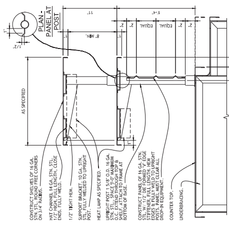
SECTION - 2-TIER ELEVATED SHELF NO SCALE REF: ITEM NO. 237
