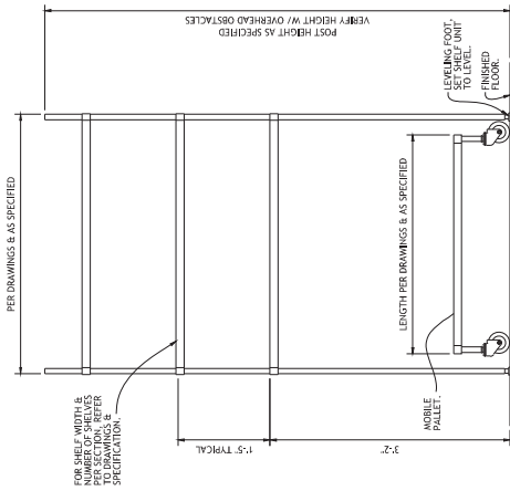
4 DETAIL - SHELVING W/ DUNNAGE RACK NO SCALE REF: ITEM NO. 044H
