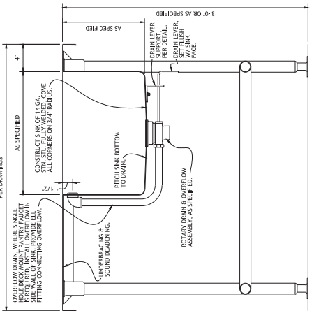
4 SECTION - TABLE W/ SINK NO SCALE REF: ITEM NO. 189Q, 238Q, 318Q & 202
