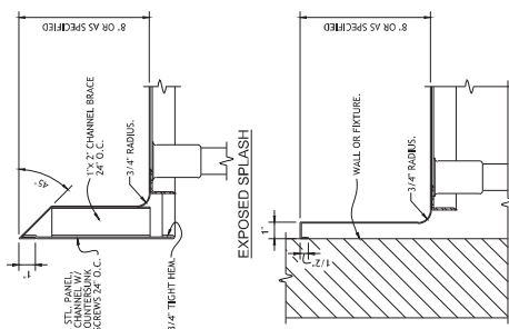
2 SECTION - TABLE TOP EDGE NO SCALE REF: ITEM NO. 0380, 3880, 4880, 51 & 154
