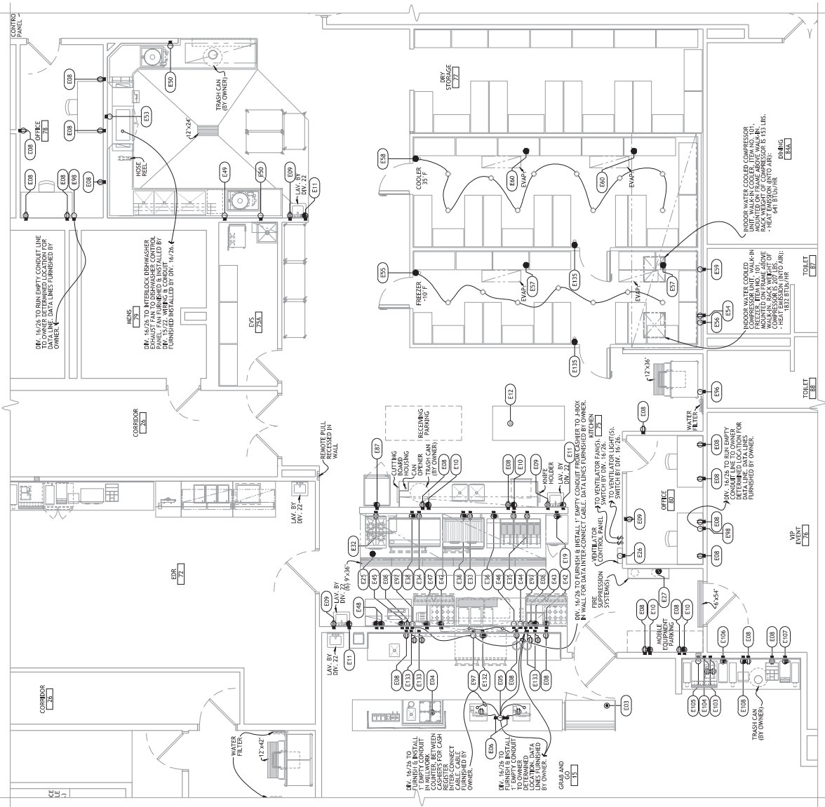
1 FOODSERVICE EQUIPMENT ELECTRICAL CONNECTION PLAN - GRAB-N-GO KITCHEN
