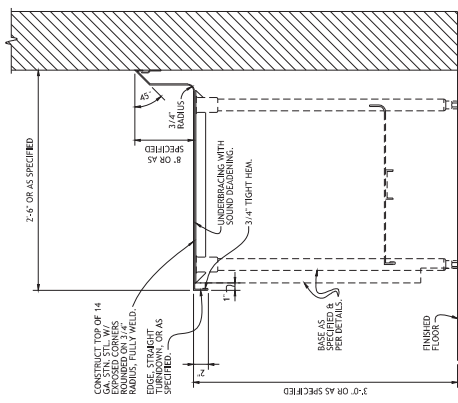
1 SECTION - TABLE/COUNTER TOP NO SCALE REF: ITEM NO. 0380, 3880, 4880, 51 & 154 980, 990, 108, 123, 124, 125, 151, 154, 203, 205, 207, 215, 237, 246, 247, 253 & 261
