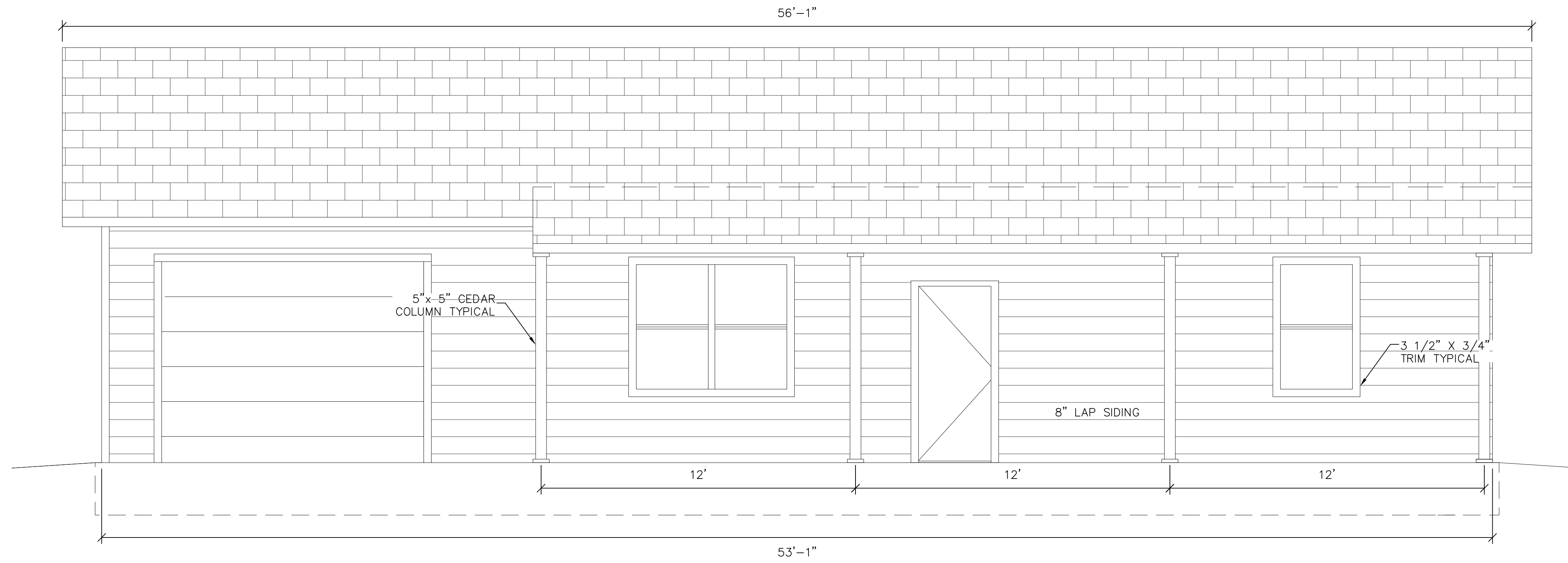
FRONT ELEVATION
