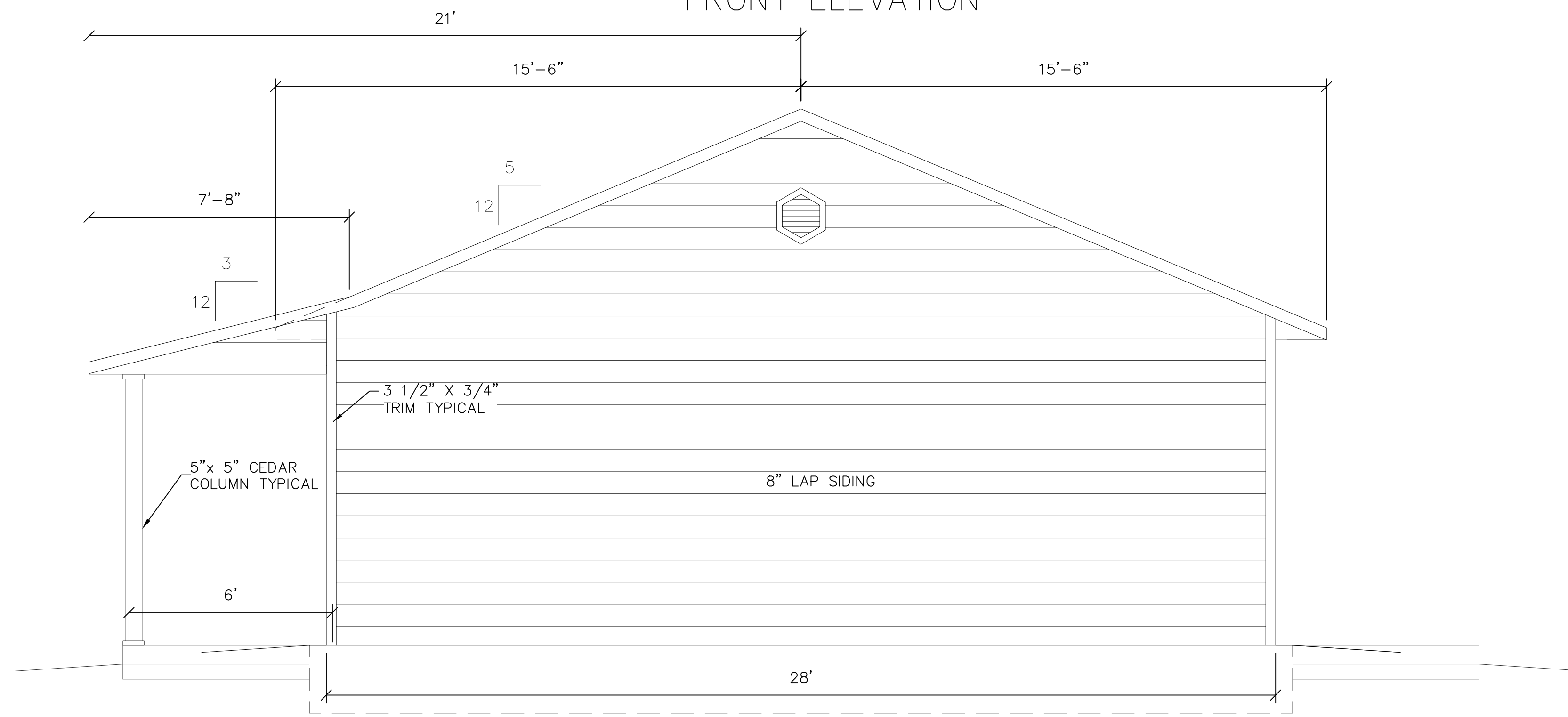
SIDE ELEVATION
