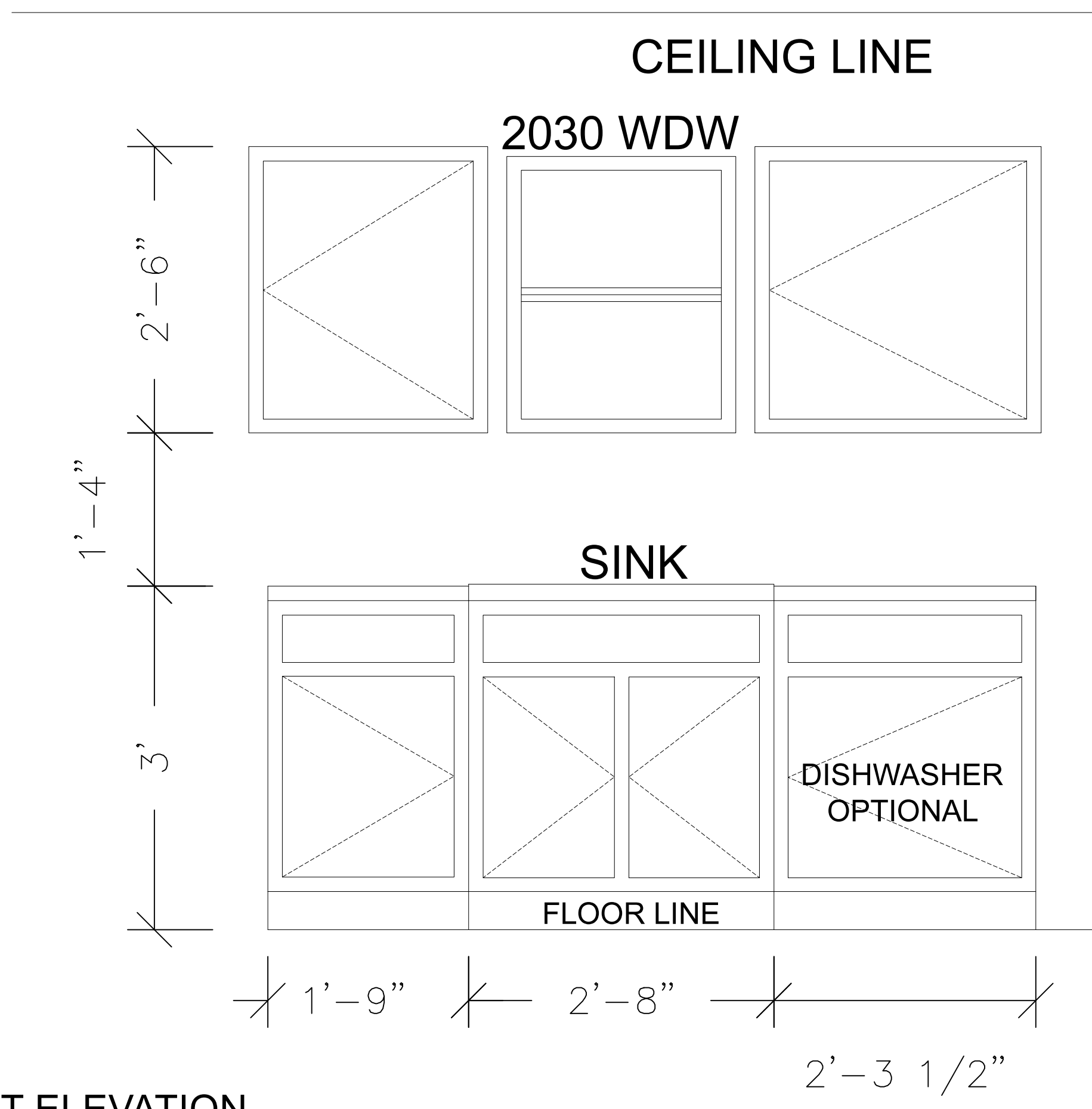
CABINET ELEVATION SCALE 1"=1'
