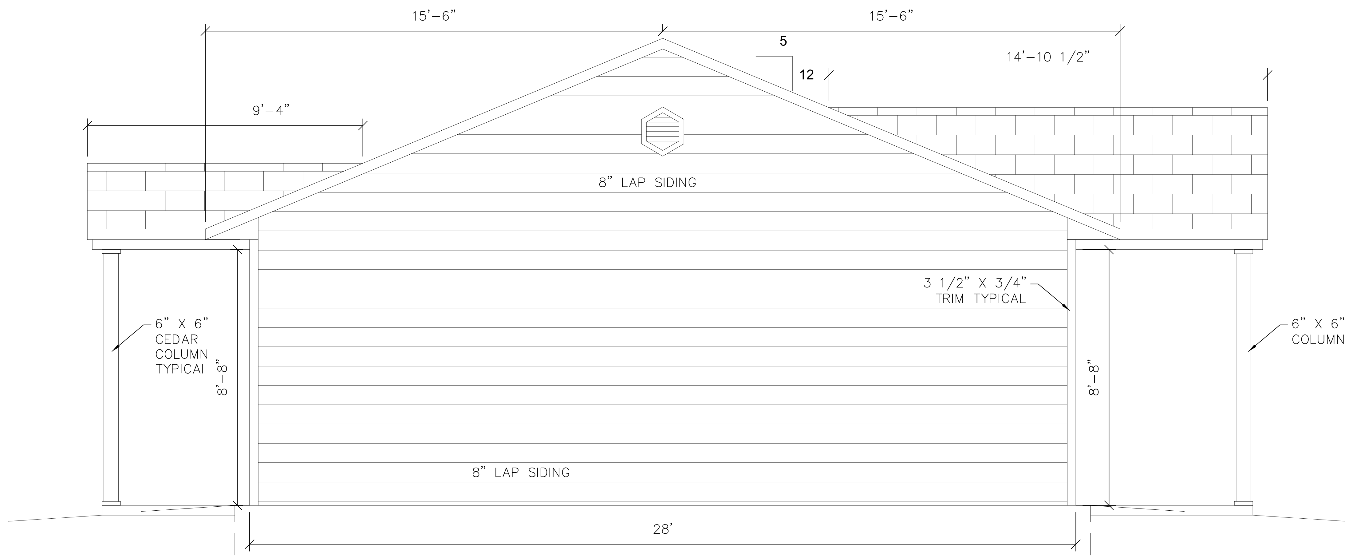
LEFT ELEVATION
