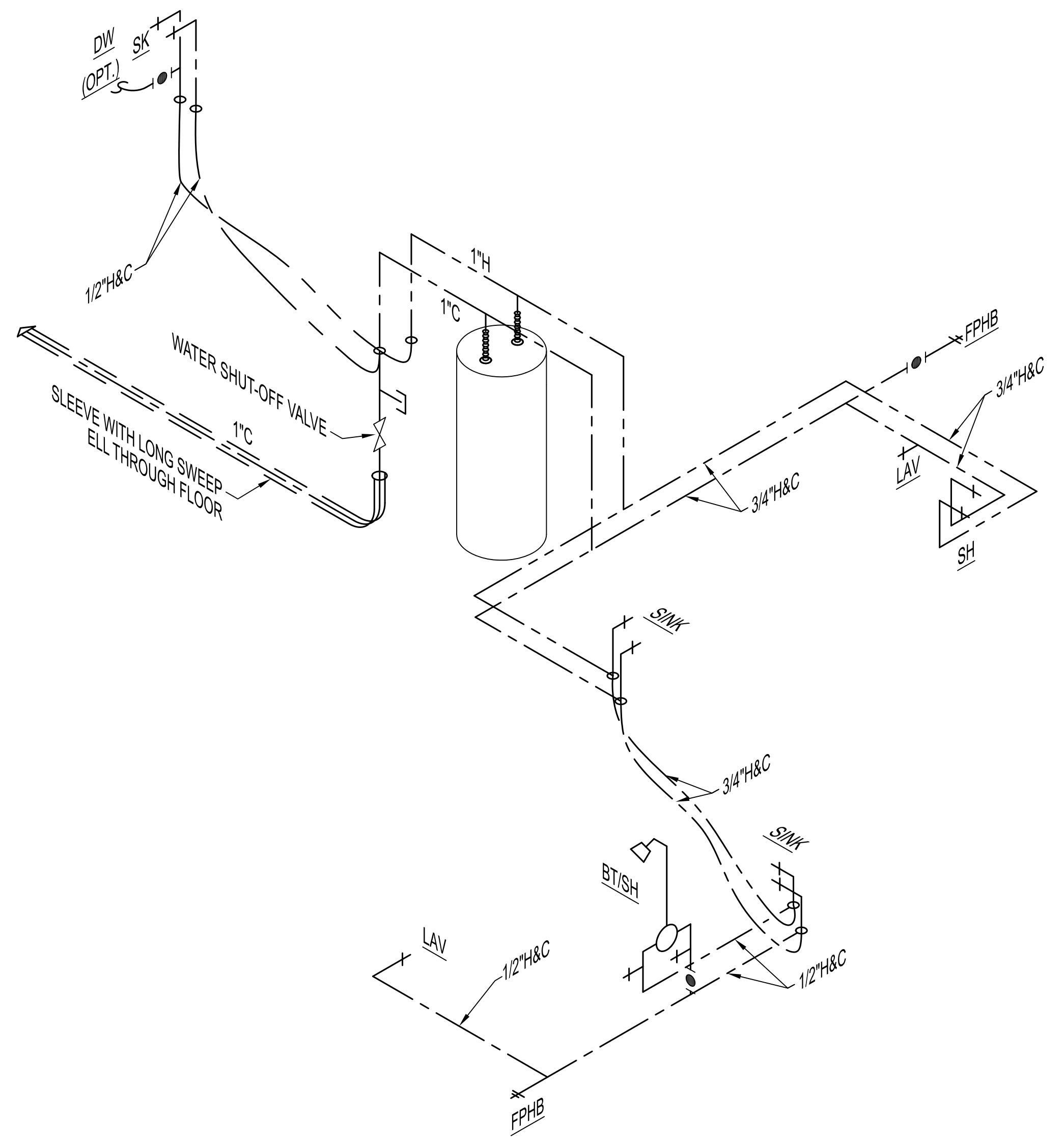
DOMESTIC WATER ISOMETRIC PLUMBING PLAN
