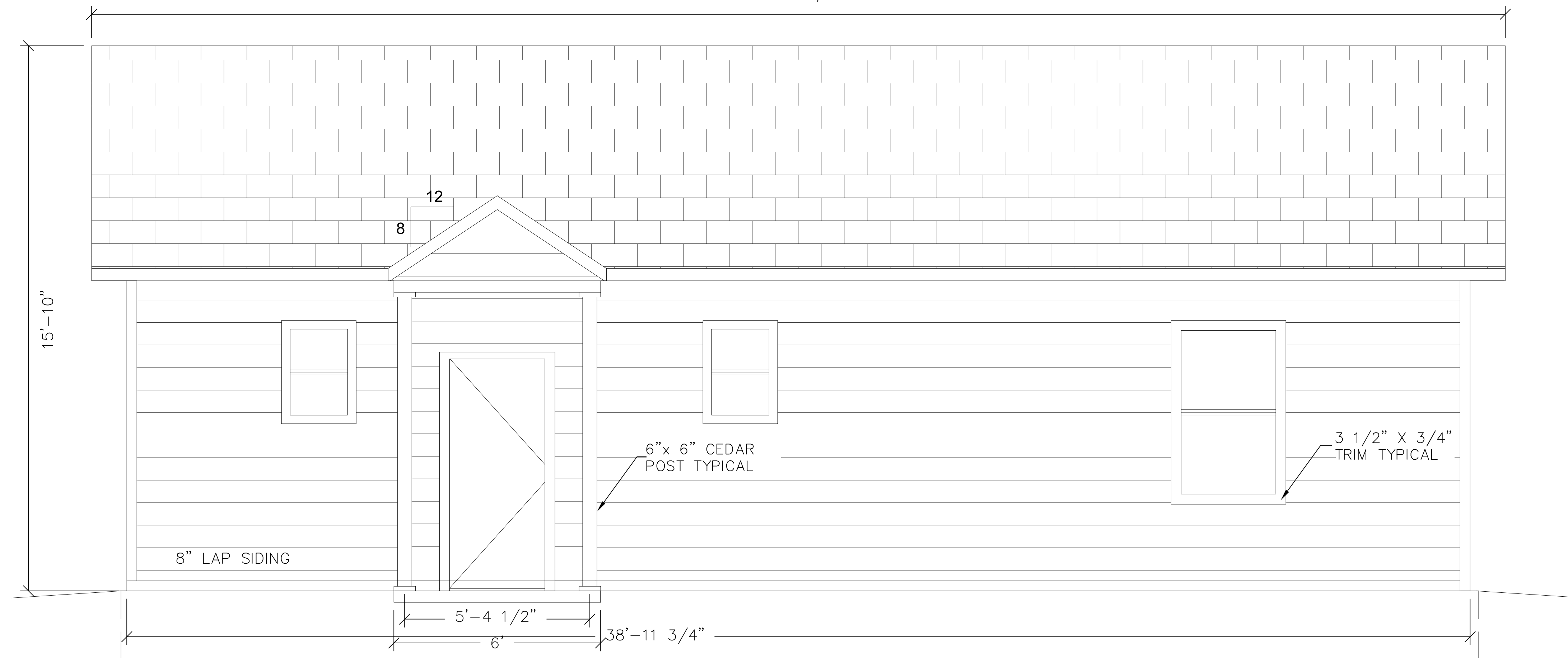
REAR ELEVATION
