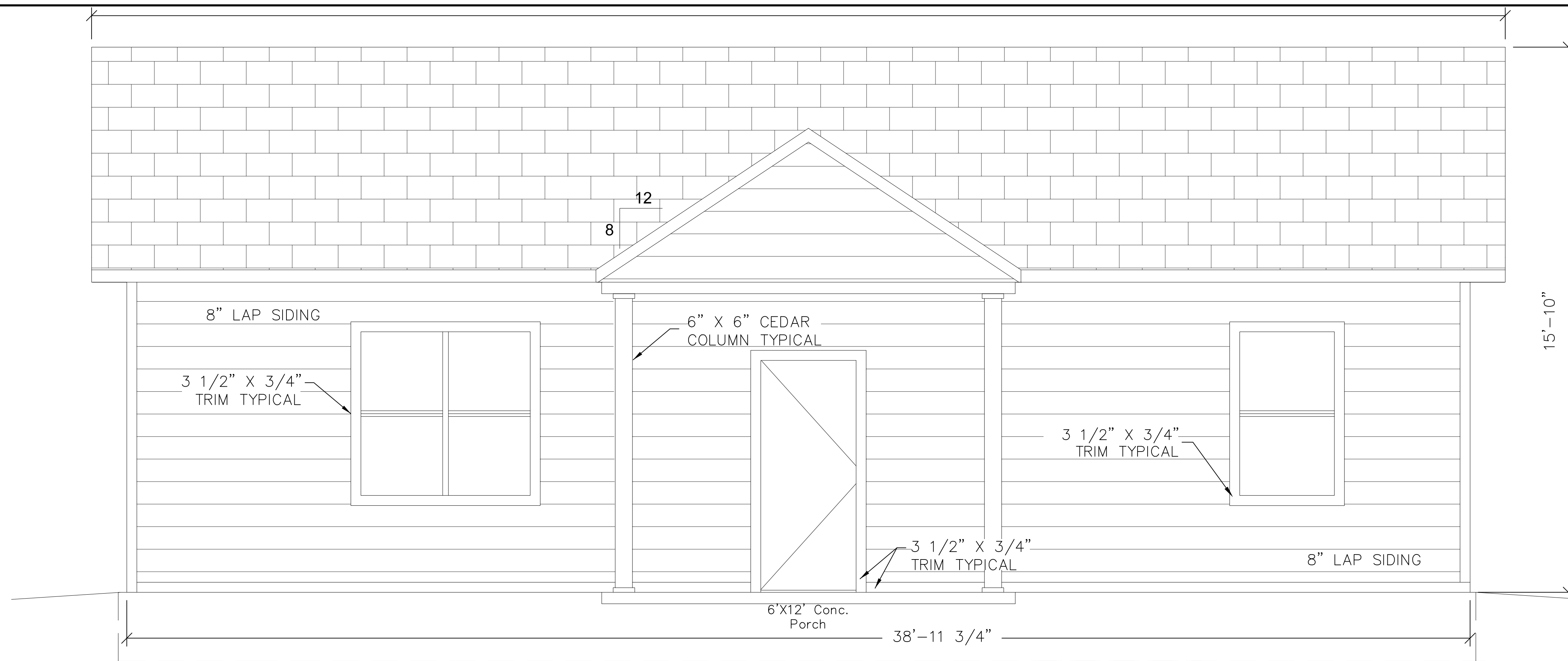
FRONT ELEVATION
