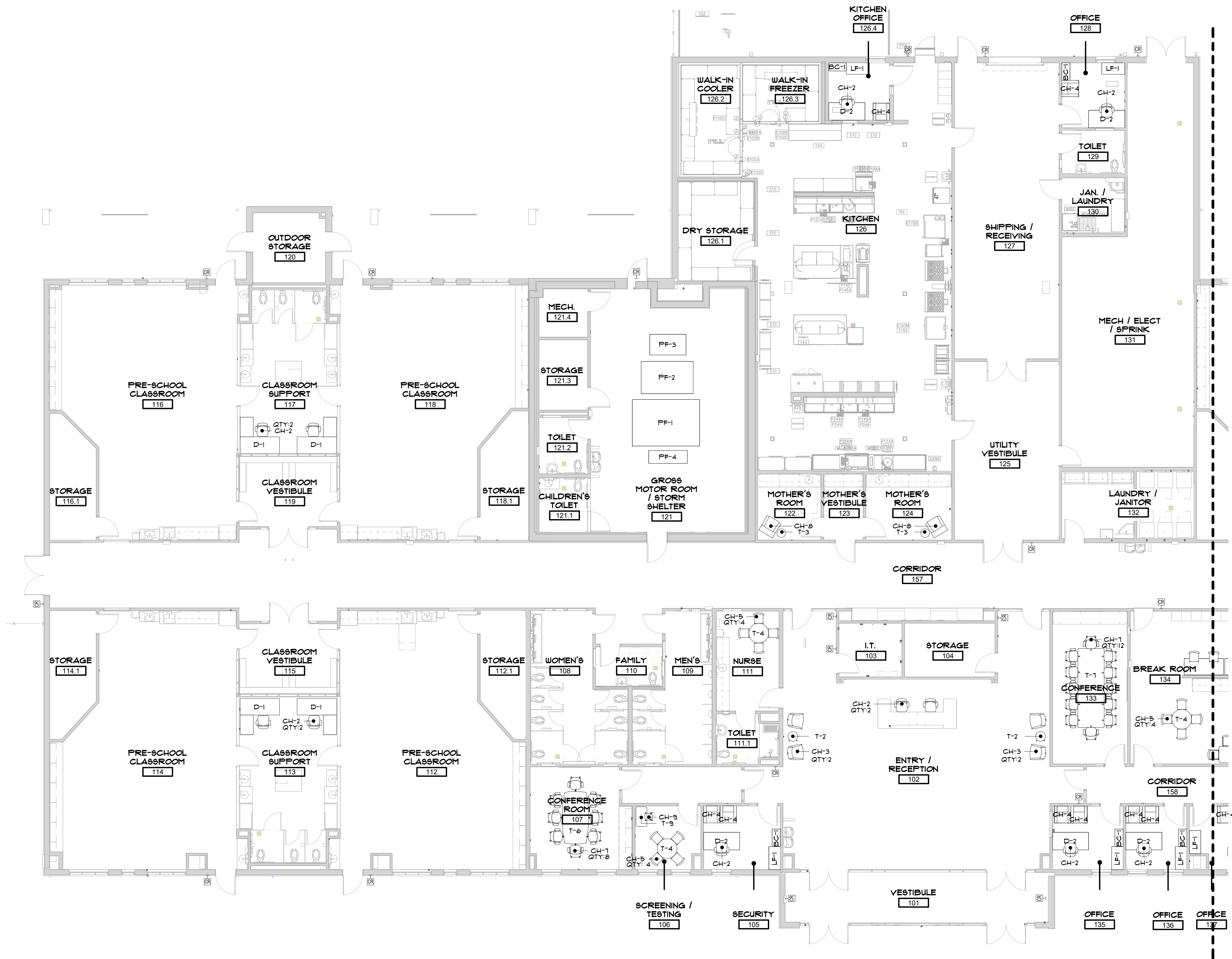
FURNITURE PLAN - AREA A
