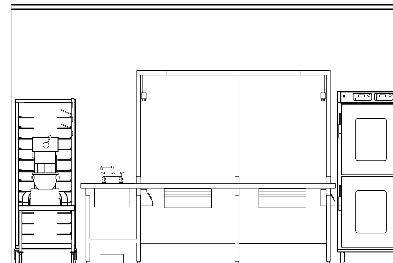
3 ELEVATION@ PREP AREA AND STAGING 1/2" = 1'-0"
