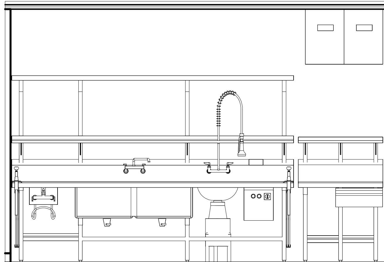
2 ELEVATION@ PREP AREA 'A' 1/2" = 1'-0"
