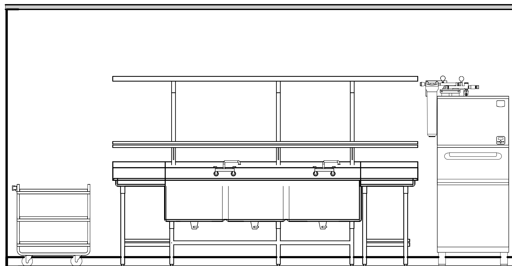
1 ELEVATION@ 2 COMP SINK 1/2" = 1'-0"
