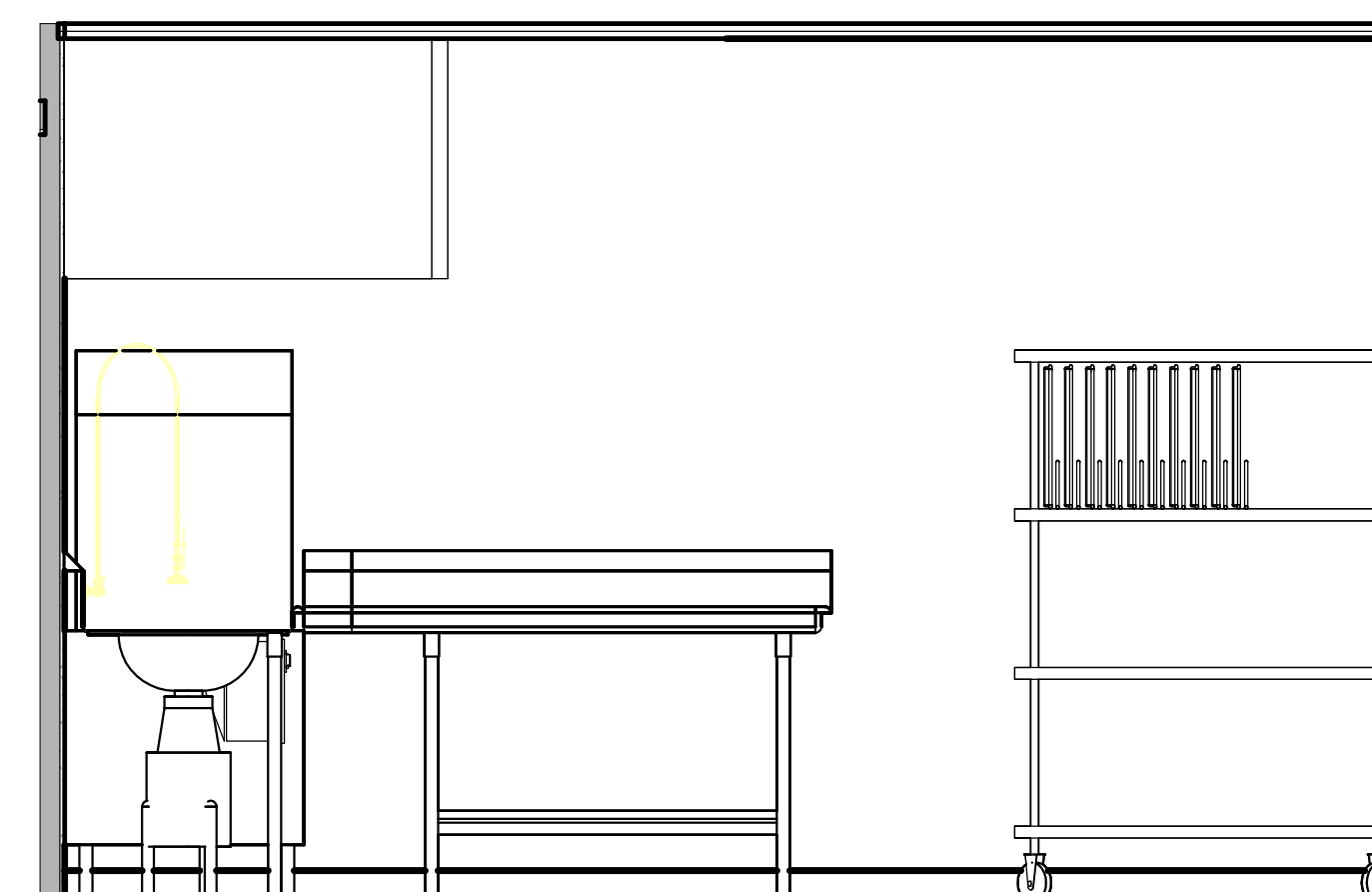
6 ELEVATION@ WAREWASH 1/2" = 1'-0"
