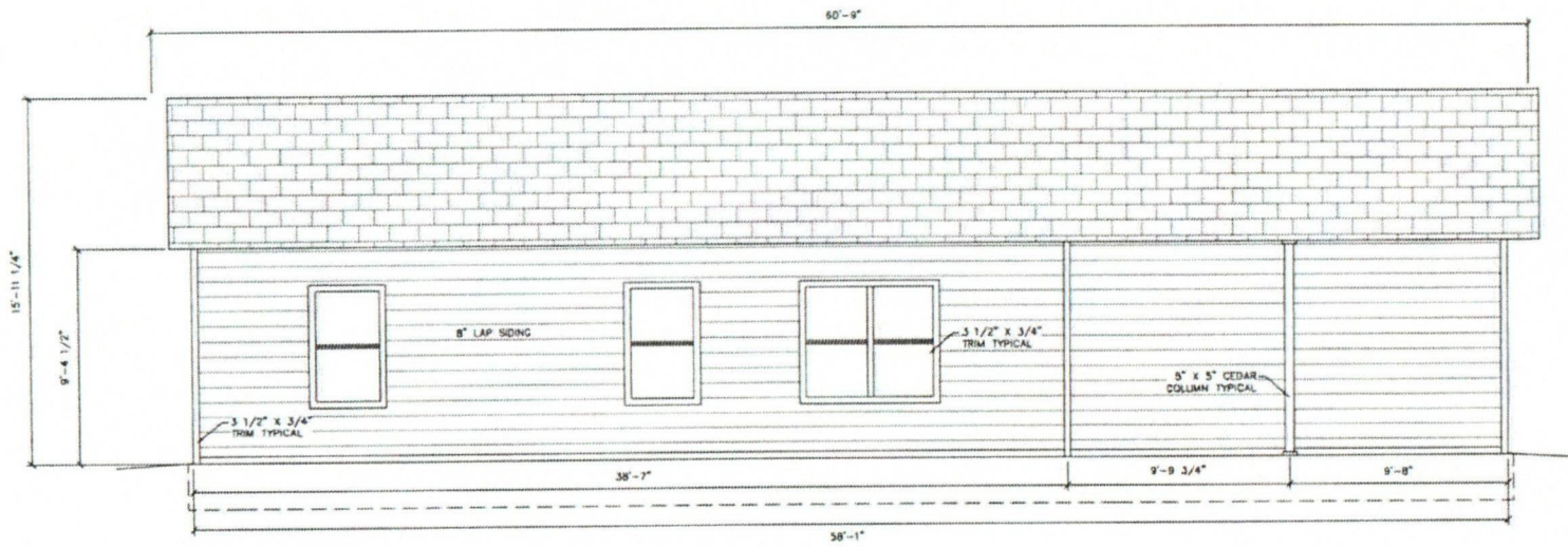
FRONT ELEVATION
