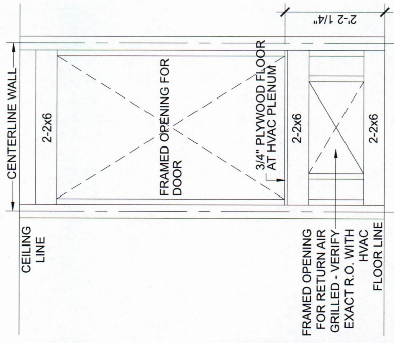
HVAC CLOSET FRAMING SCALE 1"=1 1/2"=1'
