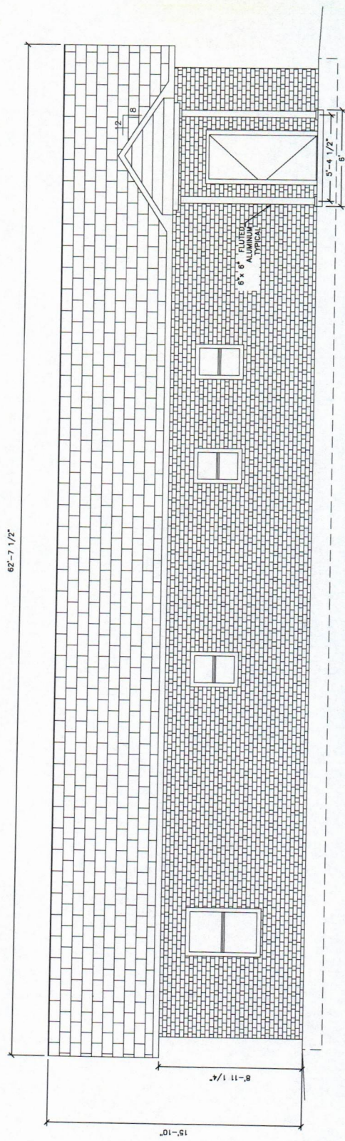
REAR ELEVATION
