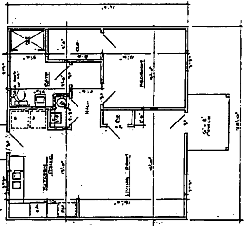
2ND FLOOR PLAN - 1/4"
