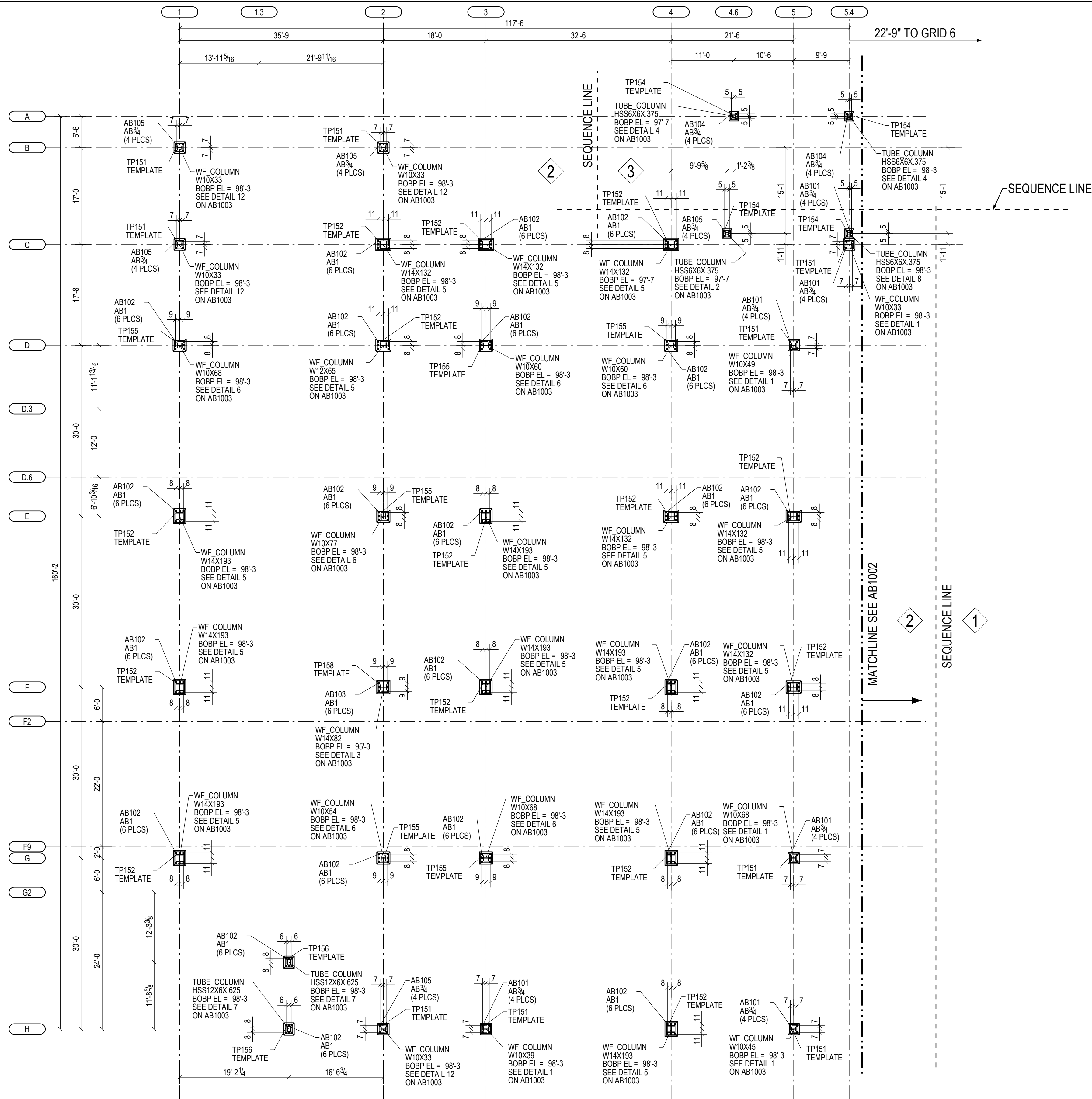
SEQ 2 & PARTIAL SEQ 3 ANCHOR BOLT PLAN
