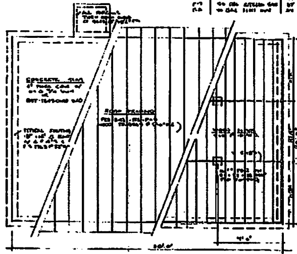
FOUNDATION / FRAMING PLAN 1/8"
