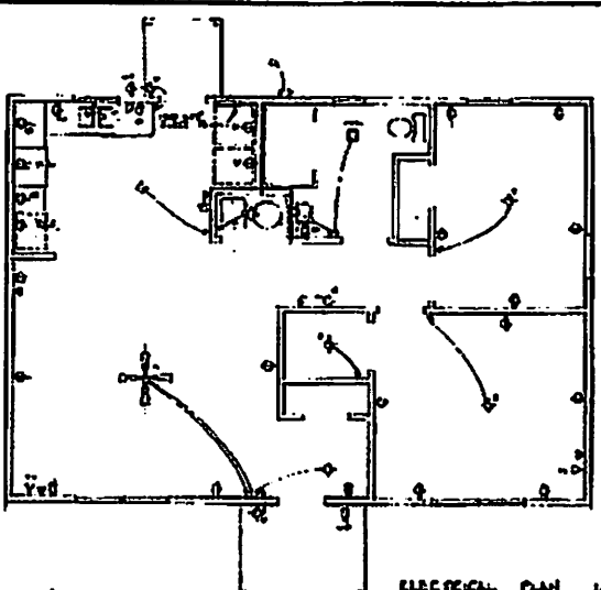
ELECTRICAL PLAN 1/8"
