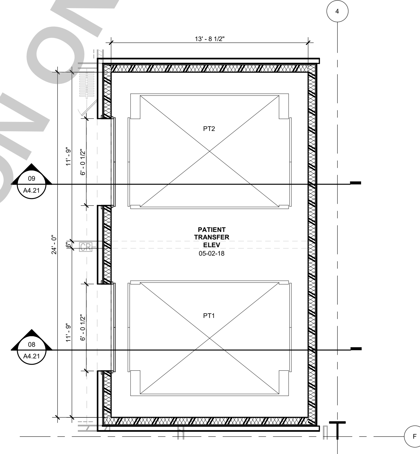
05 PATIENT TRANSFER ELEVATOR LEVEL 05 1/4" = 1'-0"
