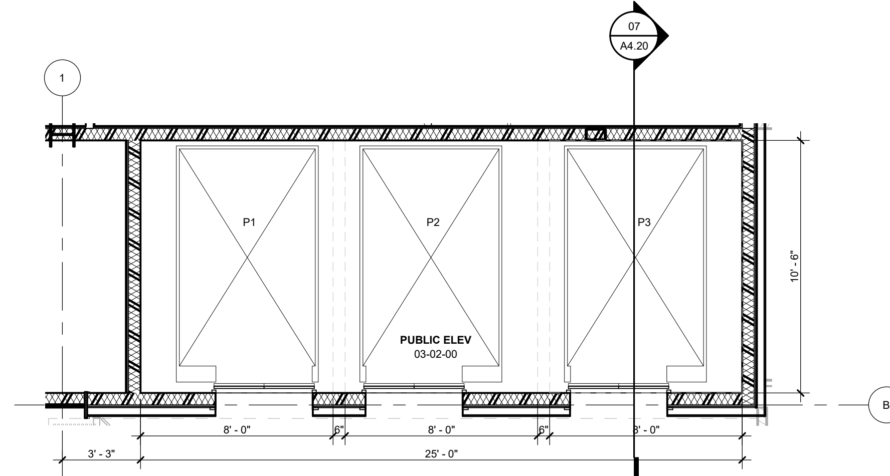
03 PUBLIC ELEVATOR LEVEL 03 SECTOR 01 1/4" = 1'-0"
