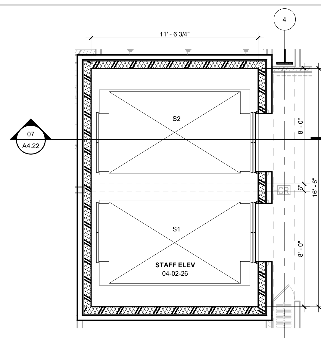
04 STAFF ELEVATOR LEVEL 04 1/4" = 1'-0"
