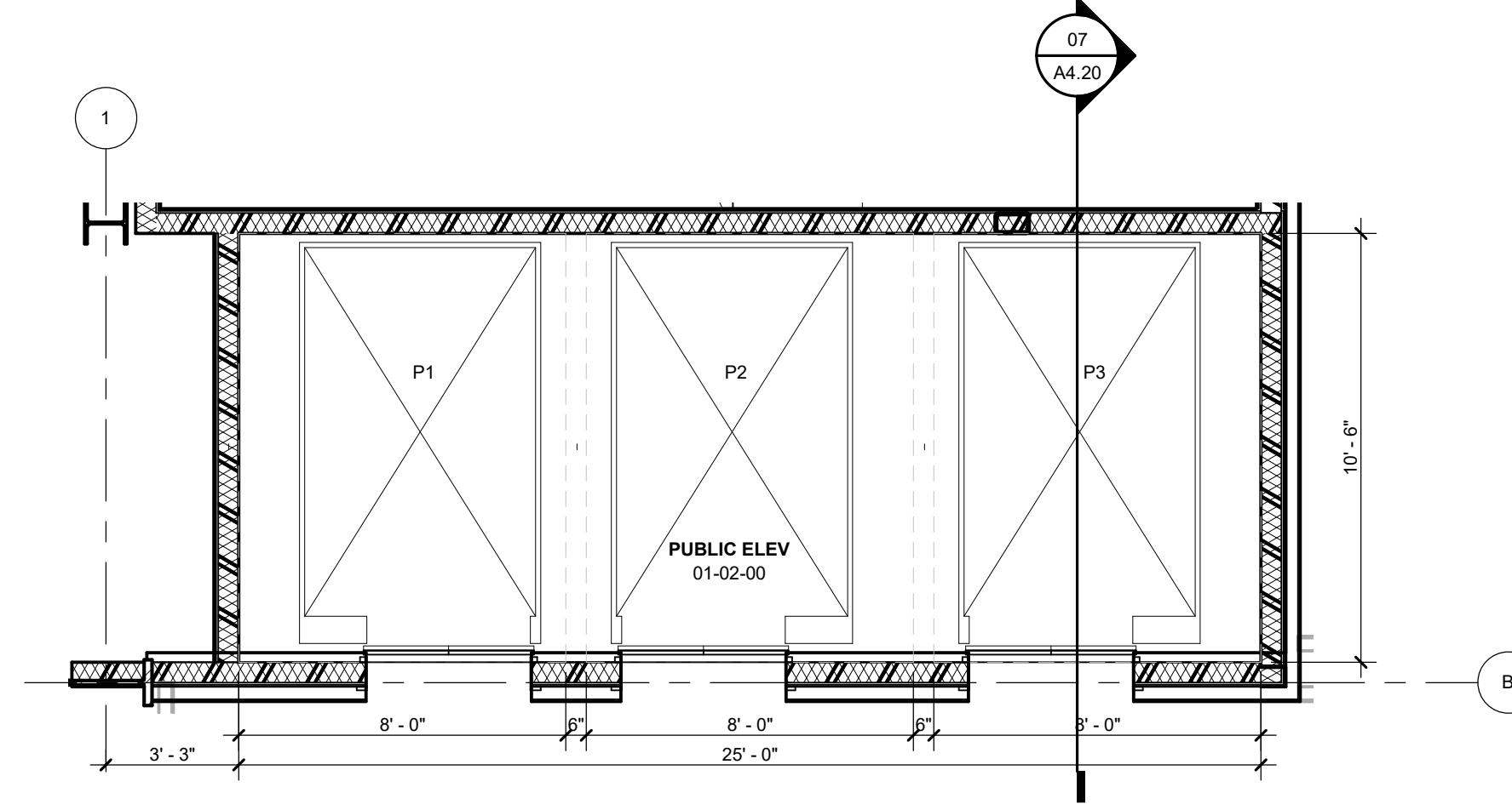
01 PUBLIC ELEVATOR LEVEL 01 SECTOR 01 1/4" = 1'-0"
