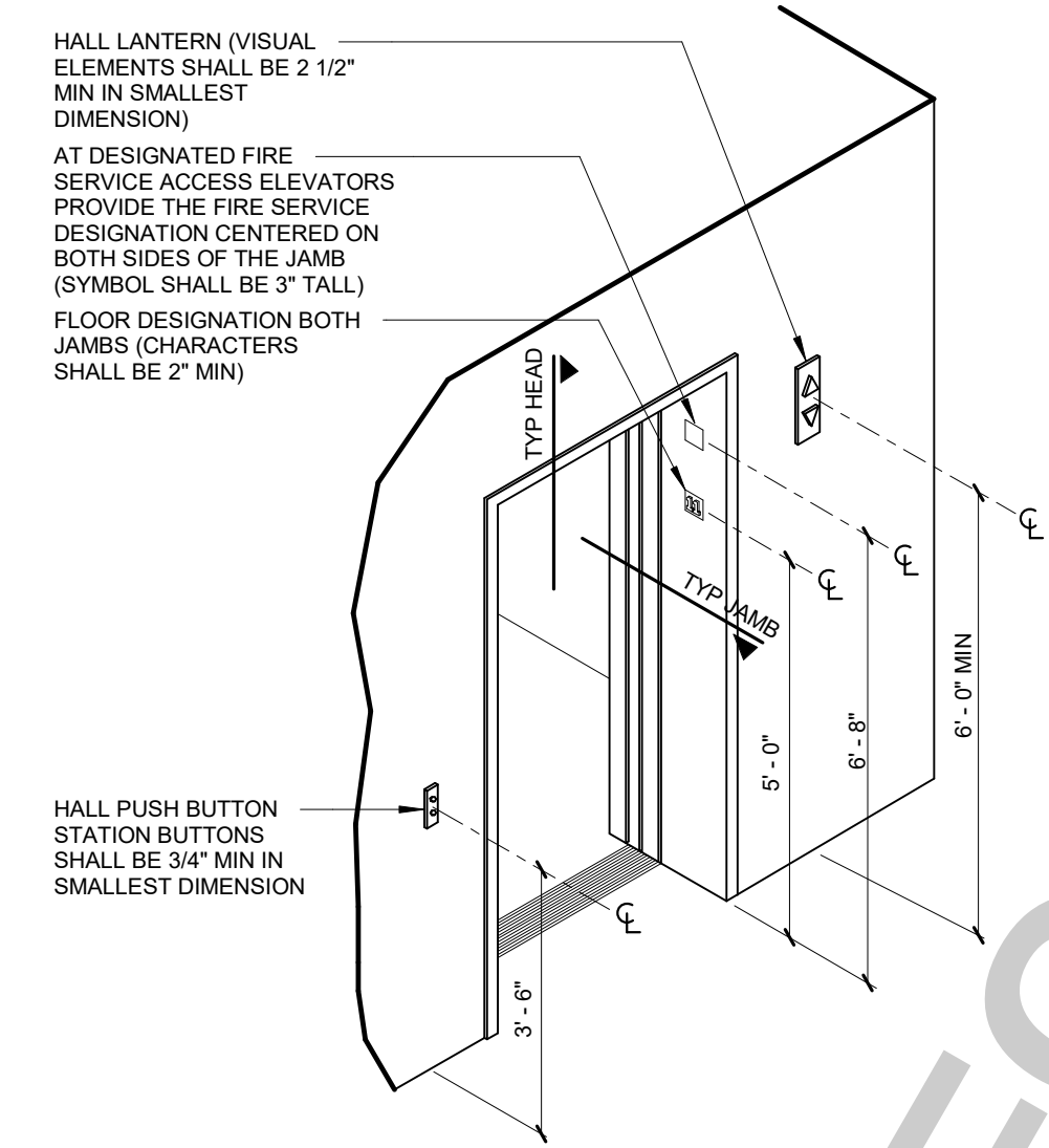
ELEVATOR ENTRY AND MOUNTING HEIGHTS NTS
