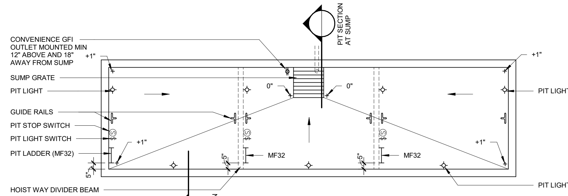
ELEVATOR PIT PLAN (TYPICAL 3 CAB) 1/4\"/>
