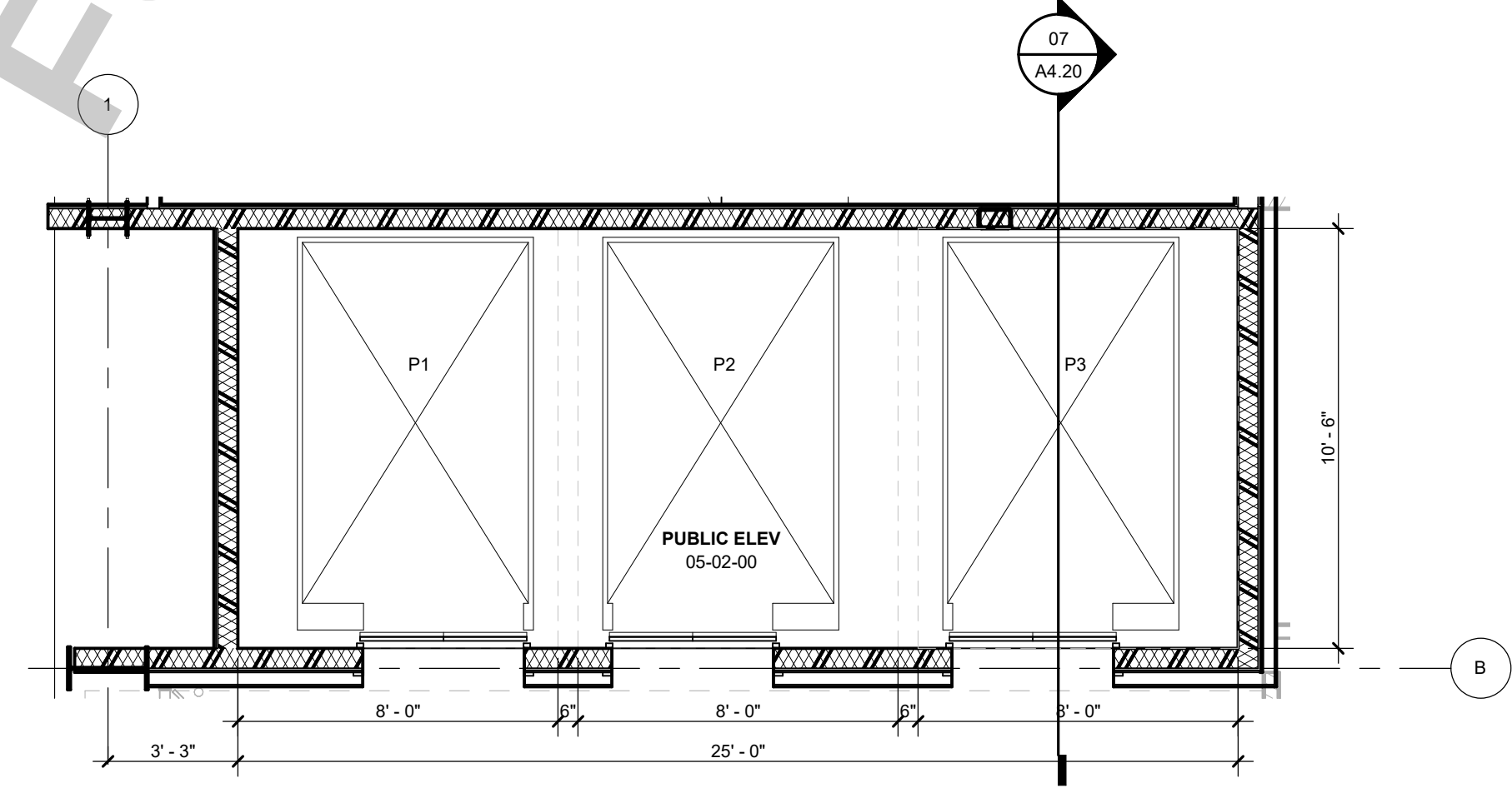
05 PUBLIC ELEVATOR LEVEL 05 SECTOR 01 1/4" = 1'-0"
