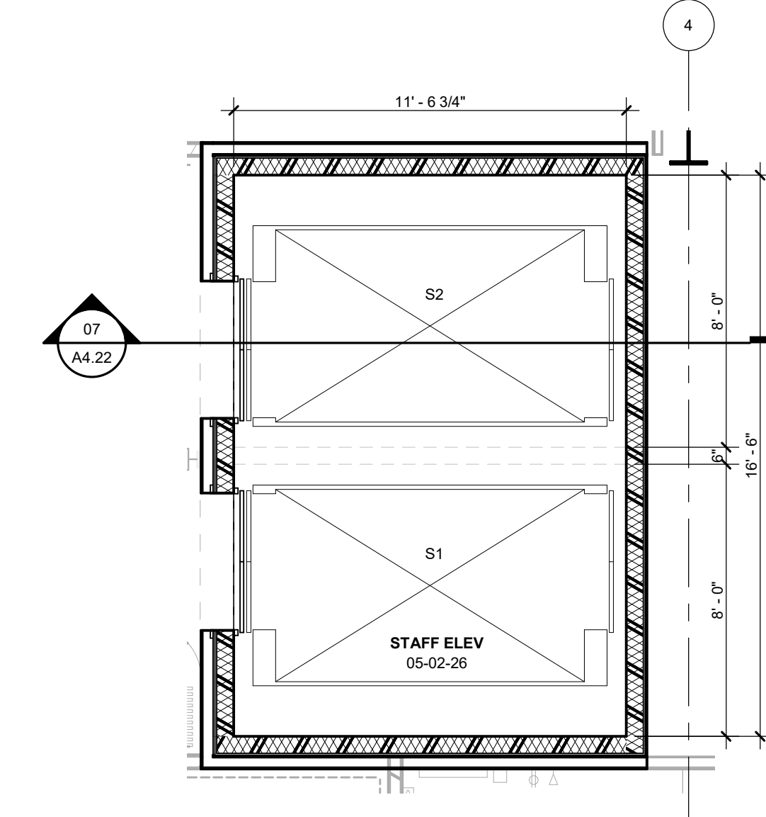
05 STAFF ELEVATOR LEVEL 05 1/4" = 1'-0"
