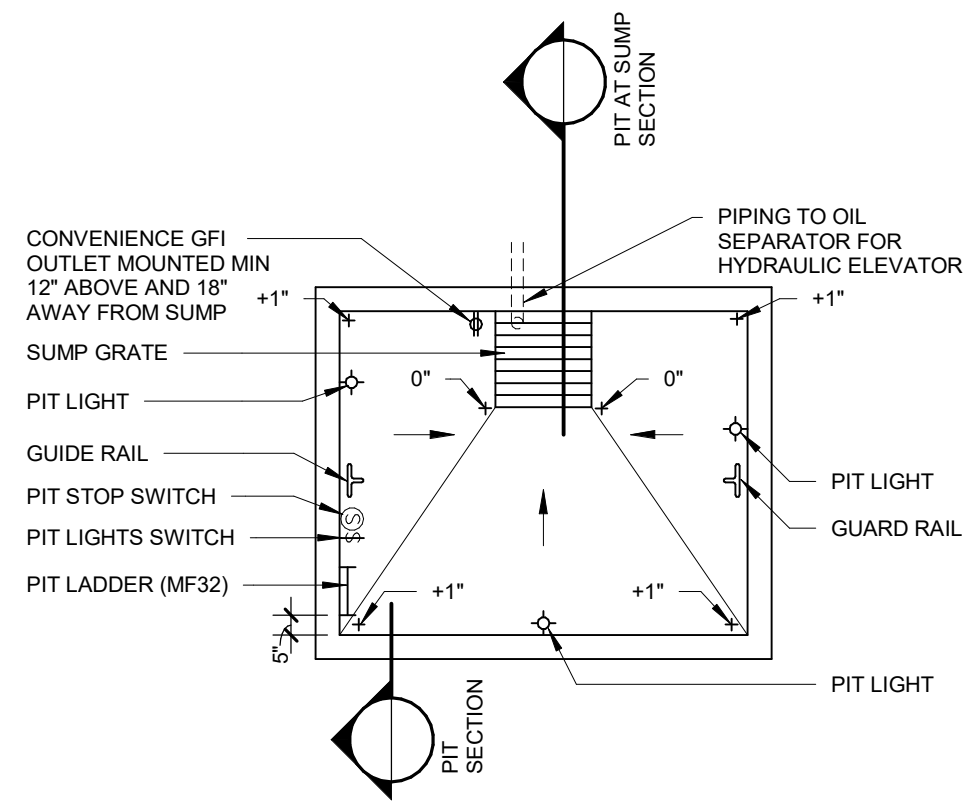
ELEVATOR PIT PLAN (TYPICAL 1 CAB) 1/4\"/>
