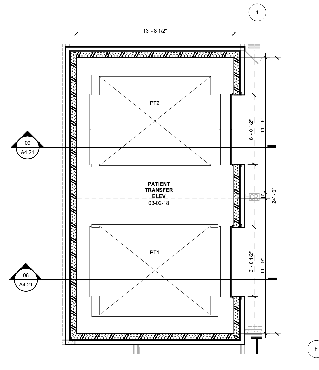
03 PATIENT TRANSFER ELEVATOR LEVEL 03 1/4" = 1'-0"
