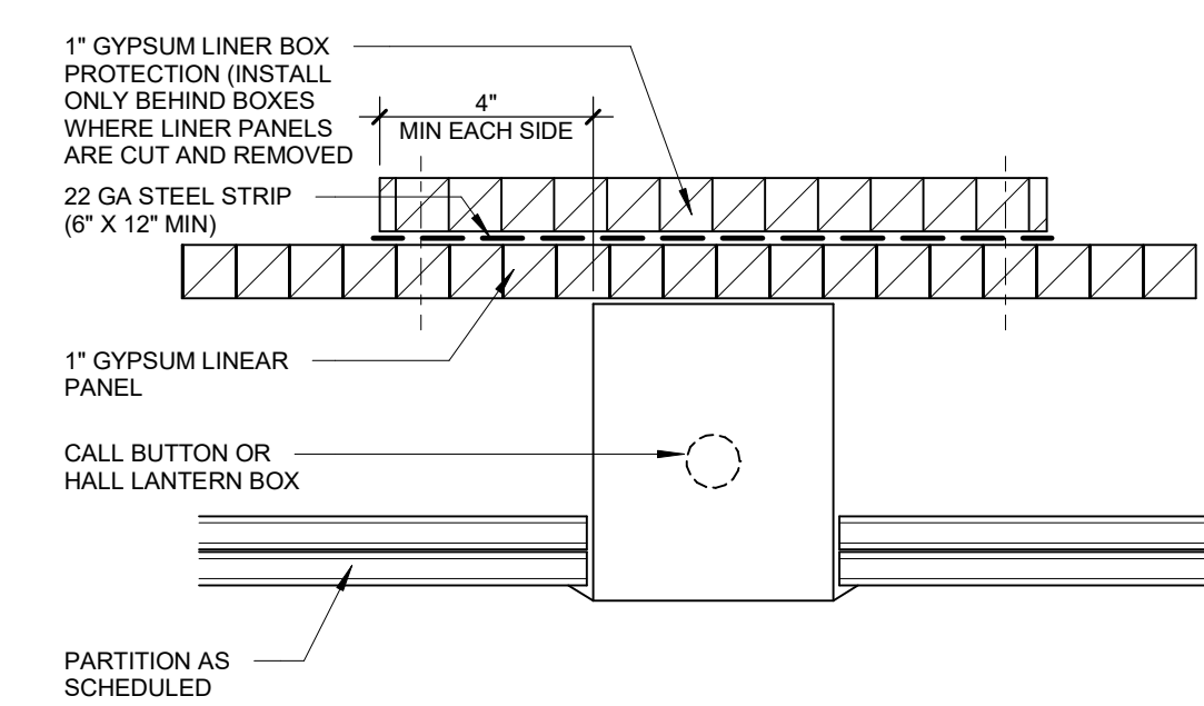
SHAFTWALL PENETRATION DETAIL AT CALL BOX AND OR HALL LANTERN 3\"/>
