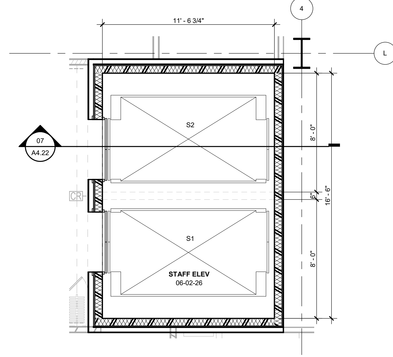
06 STAFF ELEVATOR LEVEL 06 1/4" = 1'-0"
