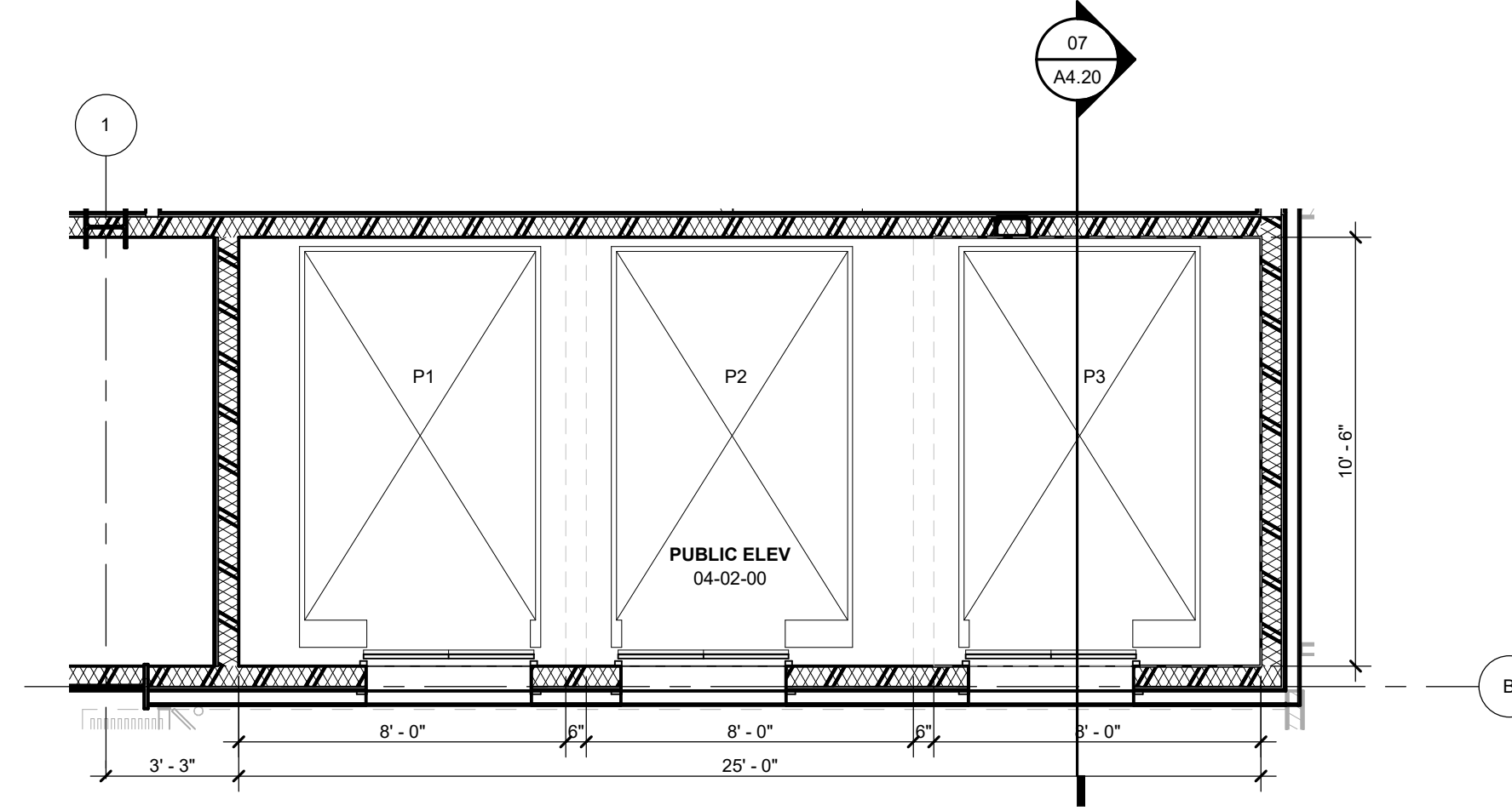
04 PUBLIC ELEVATOR LEVEL 04 SECTOR 01 1/4" = 1'-0"
