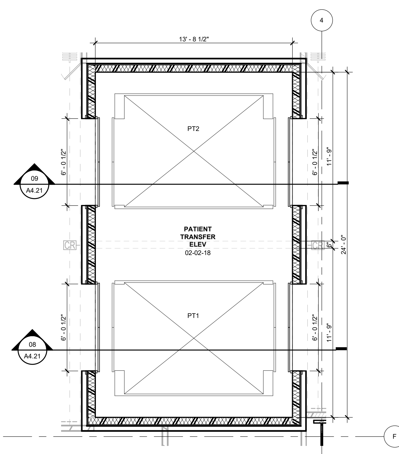
02 PATIENT TRANSFER ELEVATOR LEVEL 02 1/4" = 1'-0"
