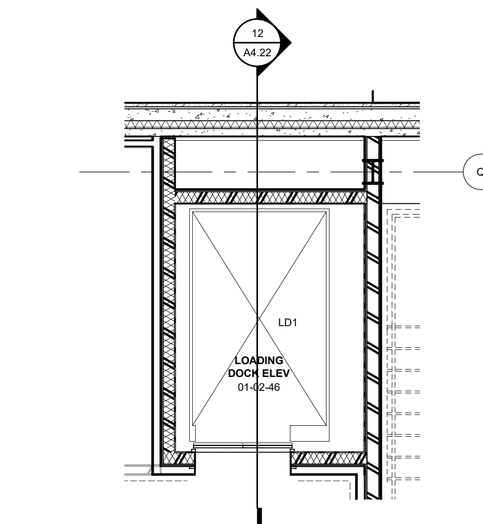
08 LOADING DOCK ELEVATOR LEVEL 01 1/4" = 1'-0"
