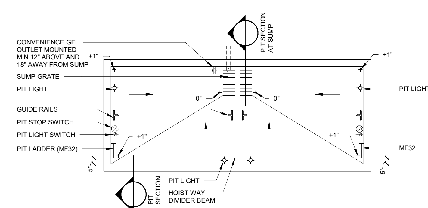
ELEVATOR PIT PLAN (TYPICAL 2 CAB) 1/4\"/>
