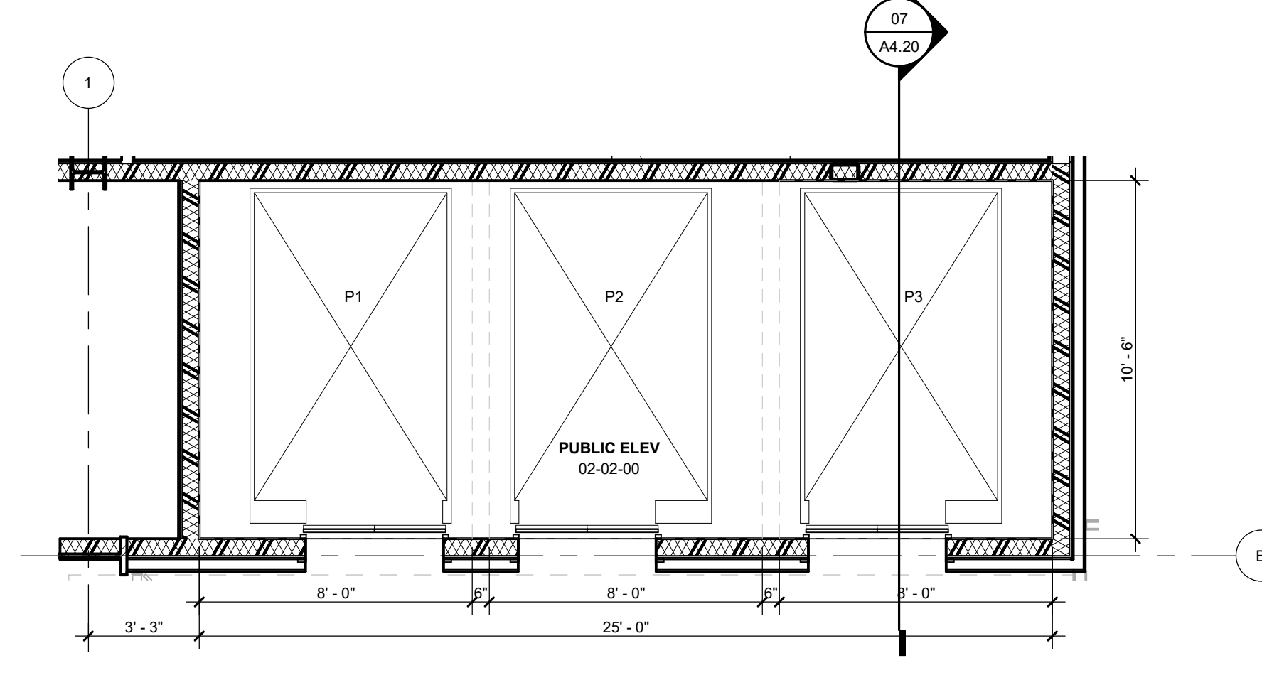
02 PUBLIC ELEVATOR LEVEL 02 SECTOR 01 1/4" = 1'-0"
