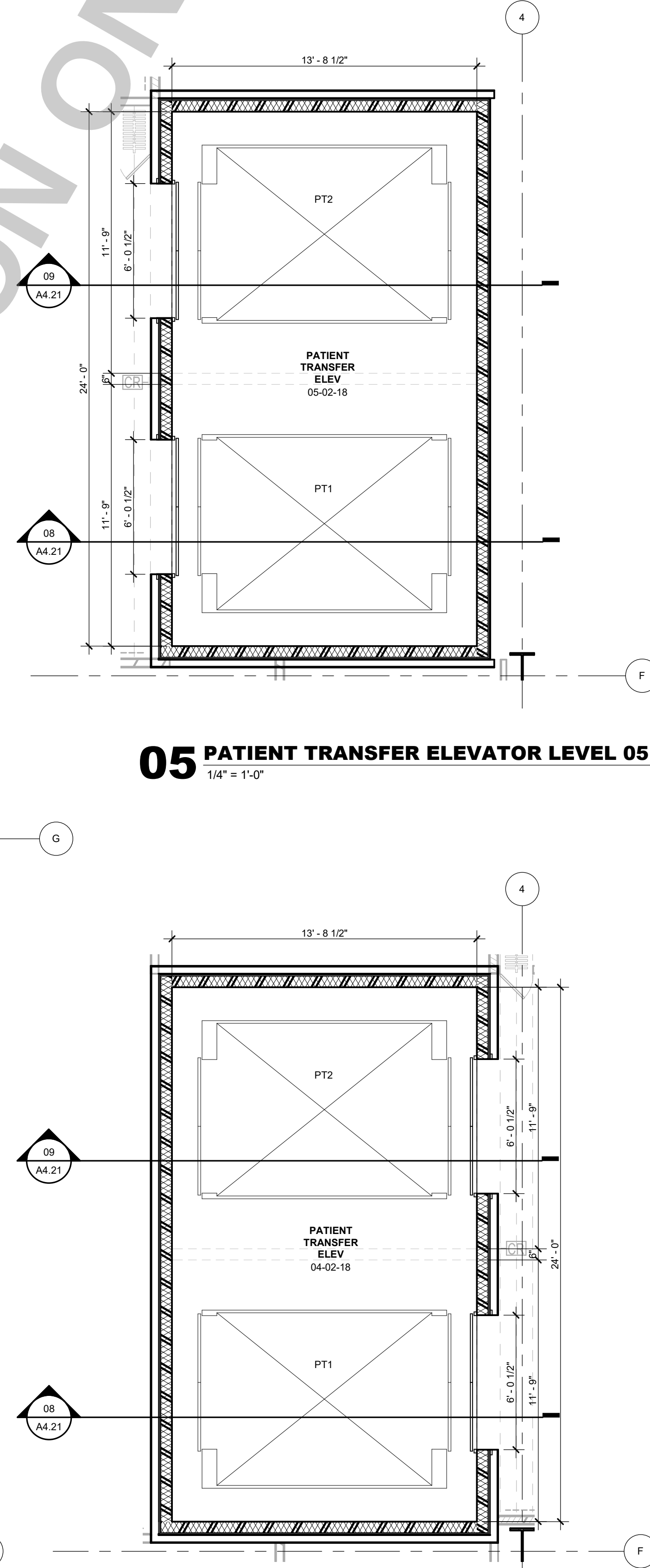
04 PATIENT TRANSFER ELEVATOR LEVEL 04 1/4" = 1'-0"
