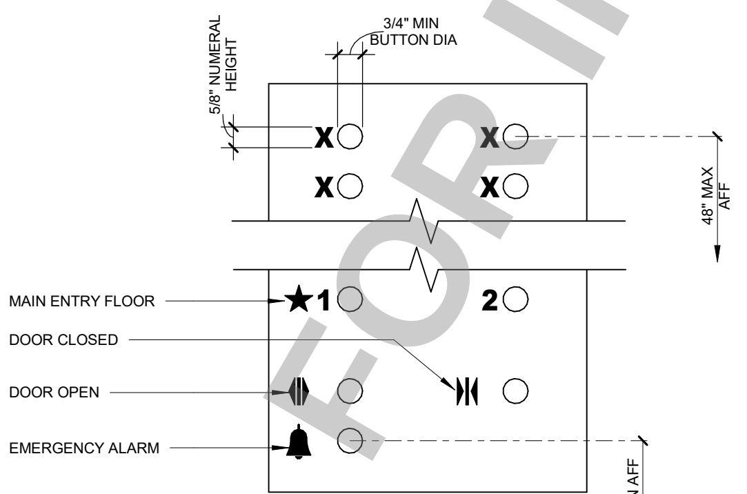
ELEVATOR PANEL DETAIL 3\"/>
