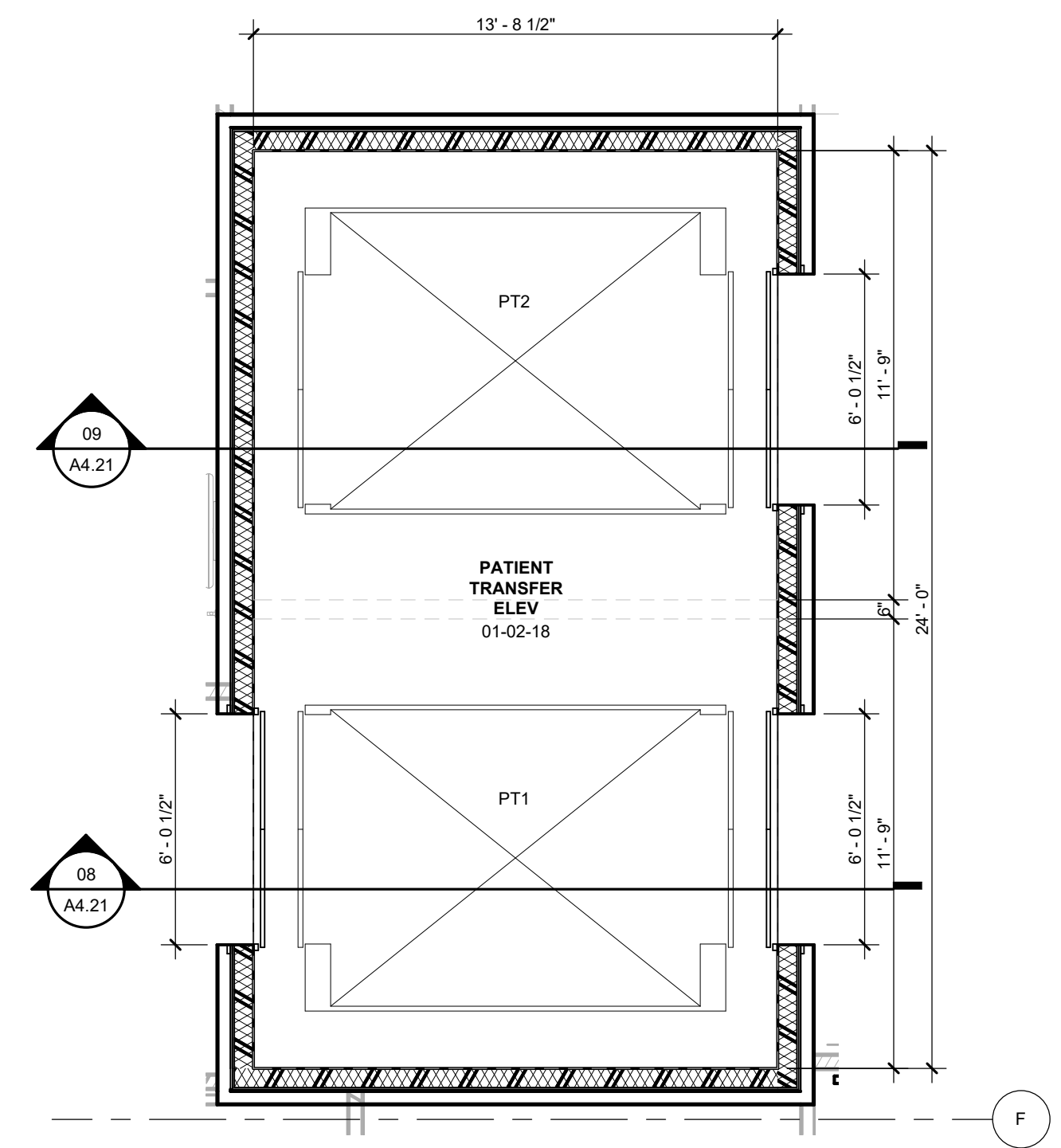
01 PATIENT TRANSFER ELEVATOR LEVEL 01 1/4" = 1'-0"
