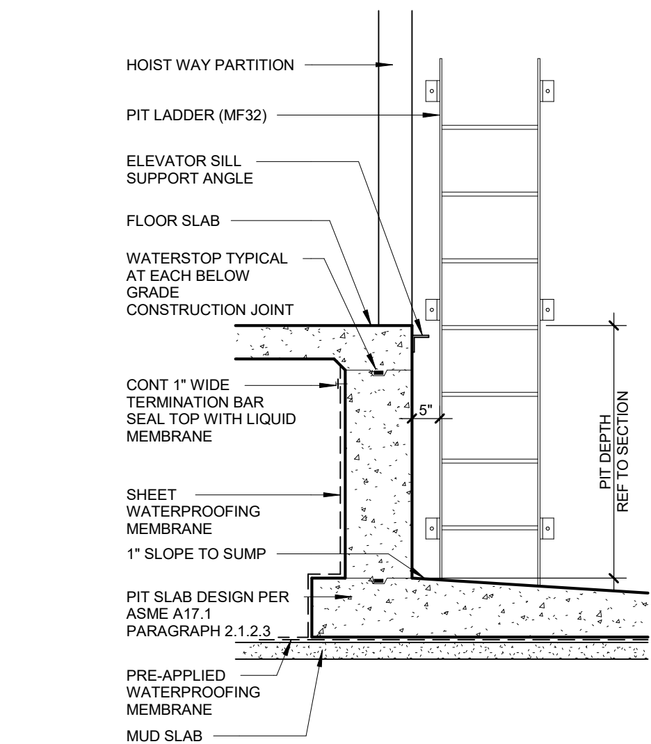
PIT SECTION WITH POSITIVE SIDE WATERPROOFING 1/2\"/>
