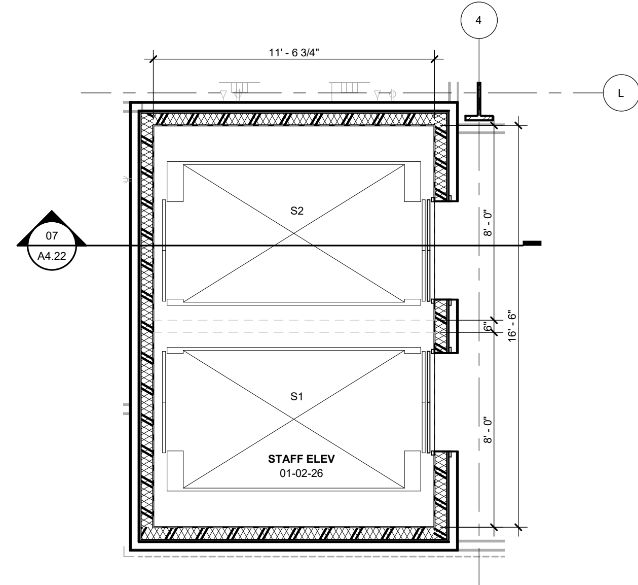
01 STAFF ELEVATOR LEVEL 01 1/4" = 1'-0"
