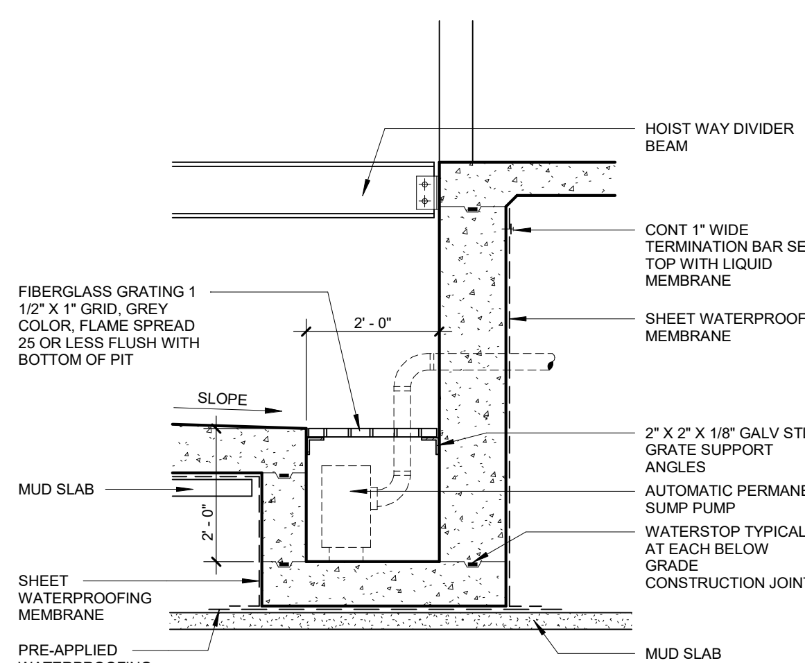
PIT SECTION AT SUMP WITH POSITIVE SIDE WATERPROOFING 1/2\"/>
