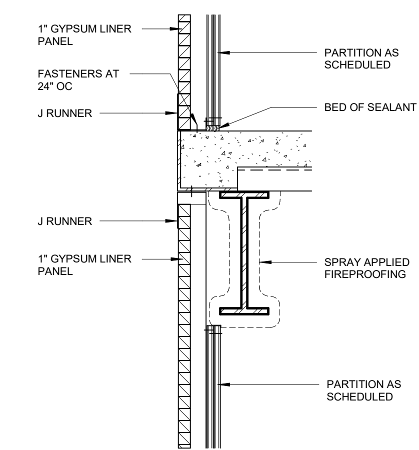
SHAFTWALL AT ELEVATOR 1 1/2\"/>
