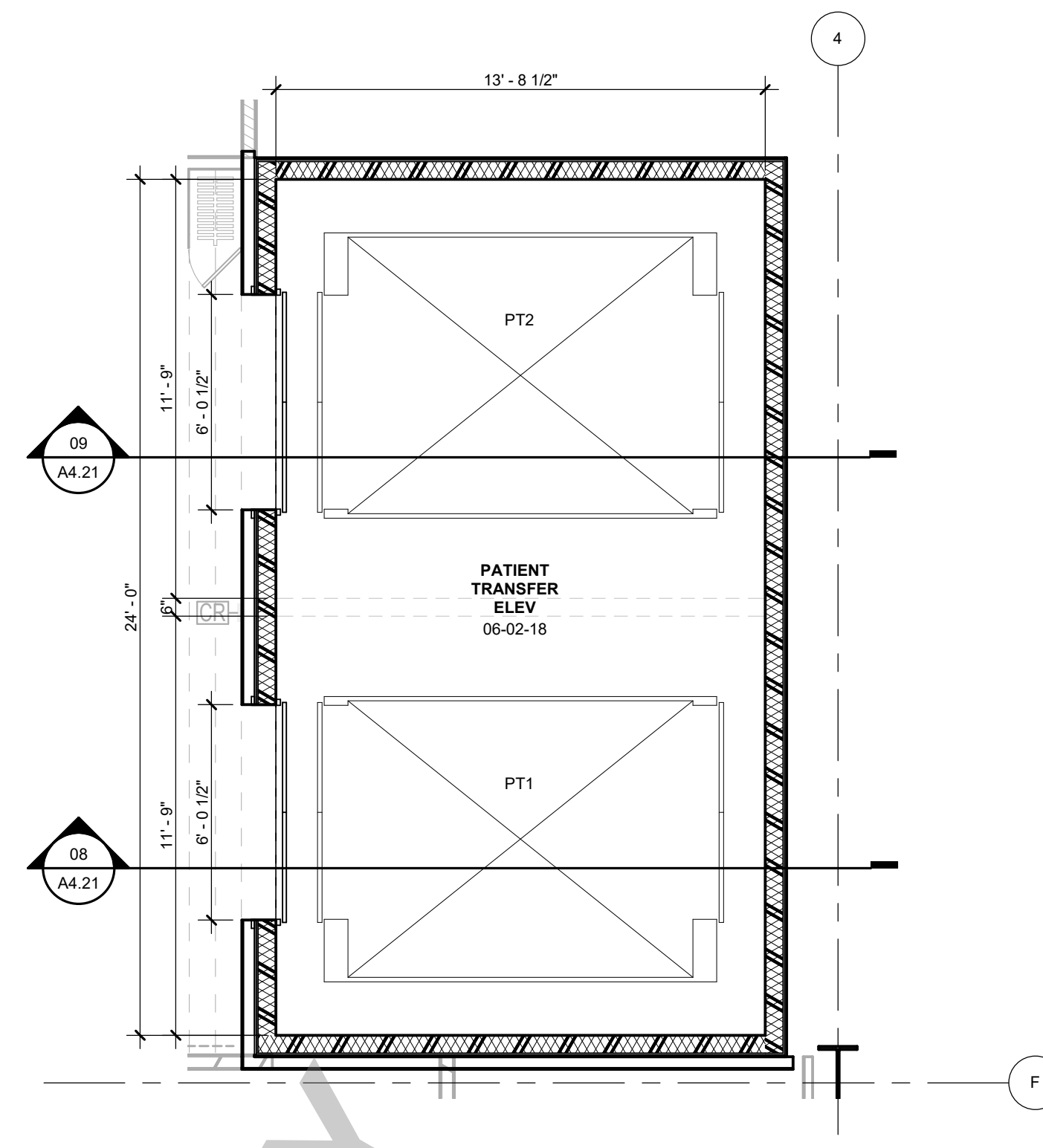
06 PATIENT TRANSFER ELEVATOR LEVEL 06 1/4" = 1'-0"
