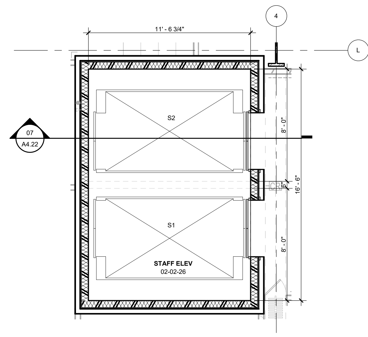
02 STAFF ELEVATOR LEVEL 02 1/4" = 1'-0"
