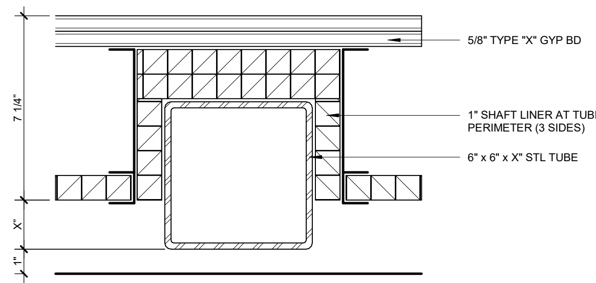
FIRE PROTECTION DETAIL AT ELEVATOR GUIDERAIL SUPPORT - STEEL TUBE GREATER THAN 4" 3\"/>
