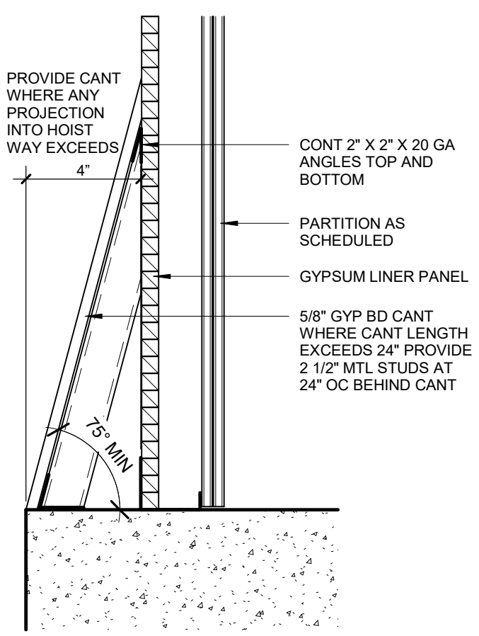
HOISTWAY DETAIL PROJECTION CANT NTS
