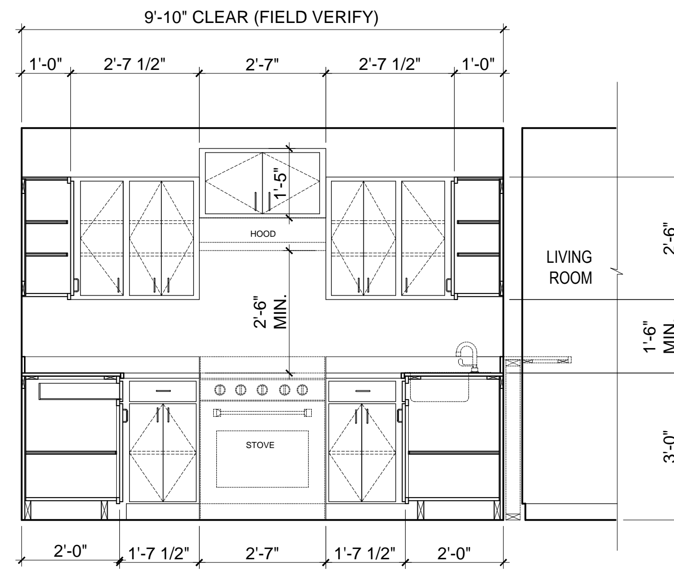
5 HOUSE 5M - KITCHEN ELEVATION SCALE: 1/2"=1'-0"
