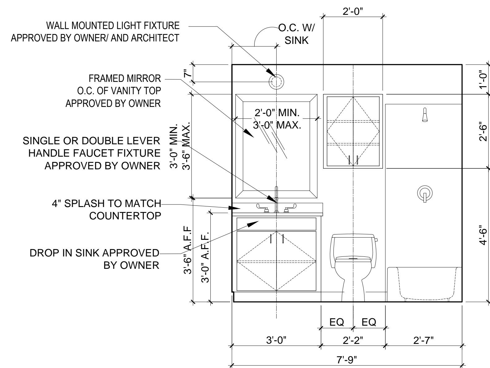
1 HOUSE 5M - MAIN BATH ELEVATION SCALE: 1/2"=1'-0"
