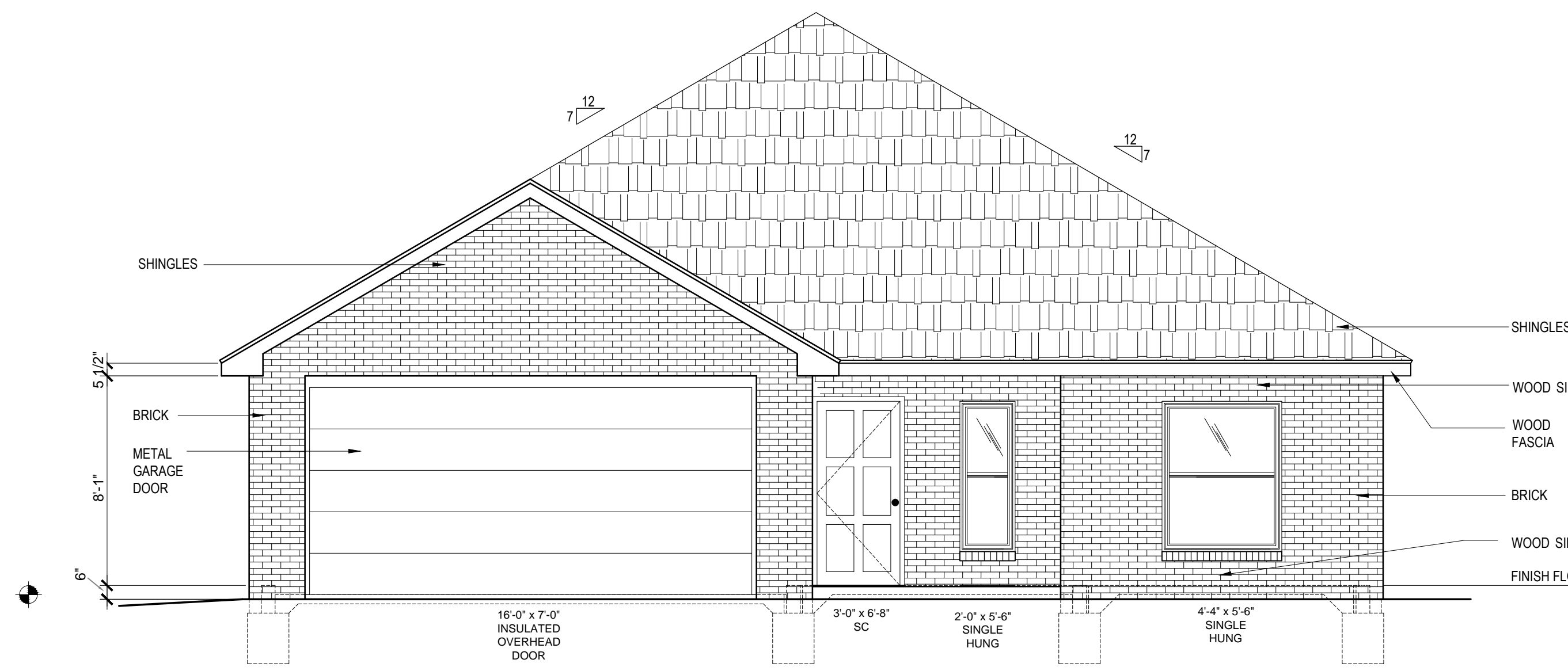
2 HOUSE 5M - FRONT ELEVATION SCALE: 1/4"=1'-0"
