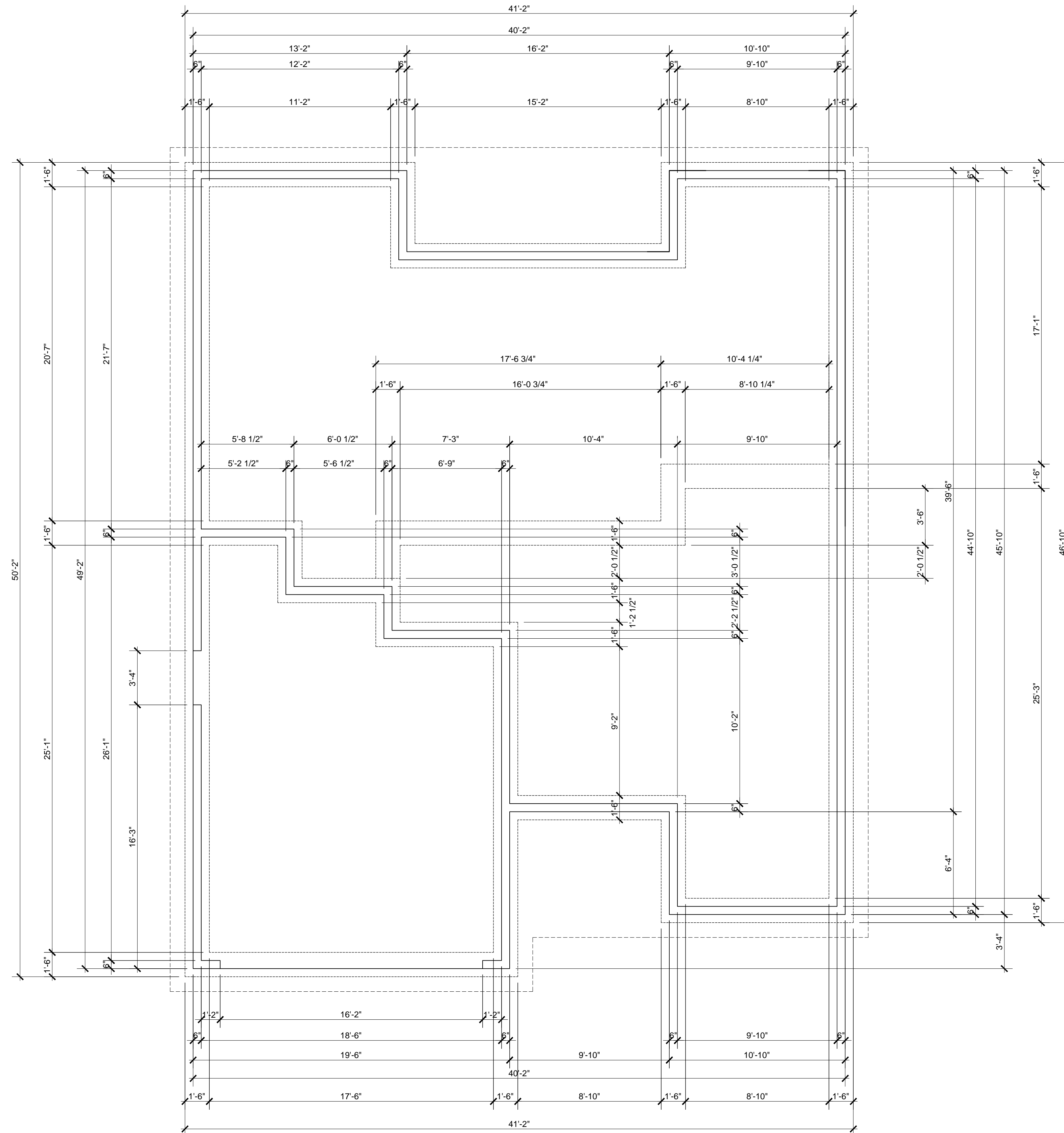
1 HOUSE 5M - FOUNDATION PLAN SCALE: 1/4"=1'-0"
