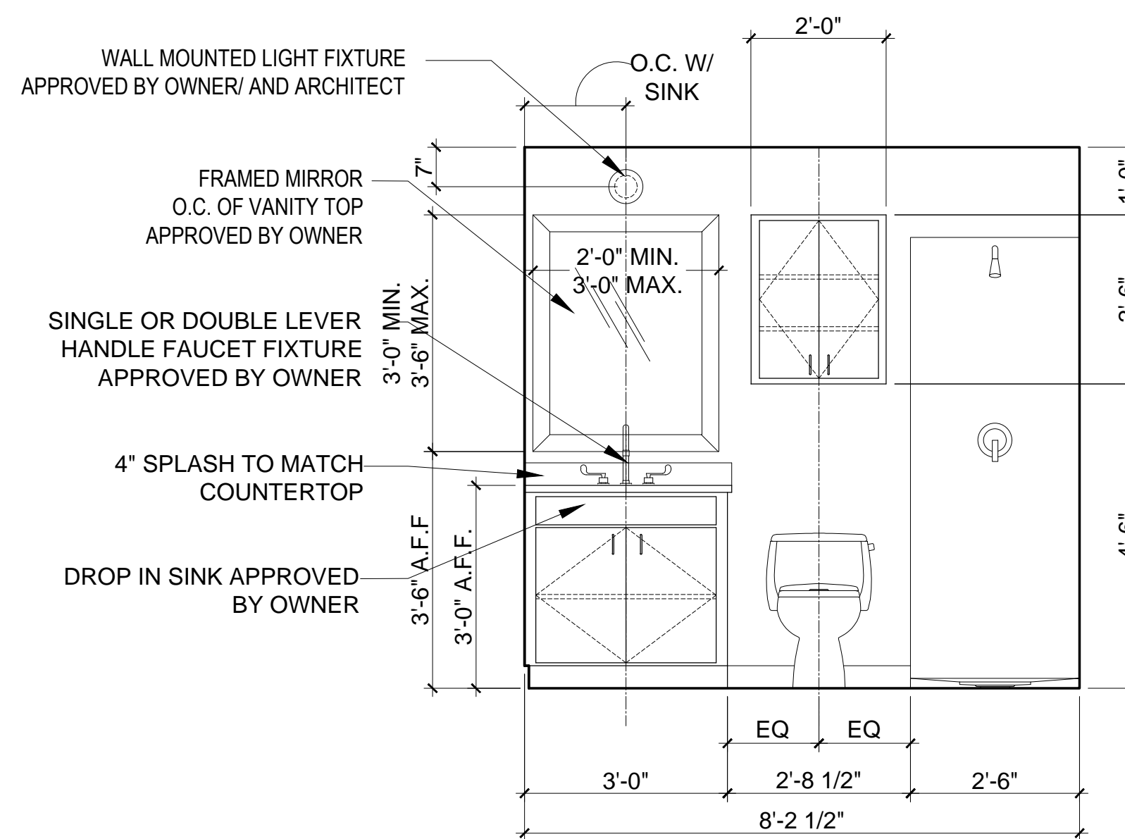
2 HOUSE 5M - MASTER BATH ELEVATION SCALE: 1/2"=1'-0"
