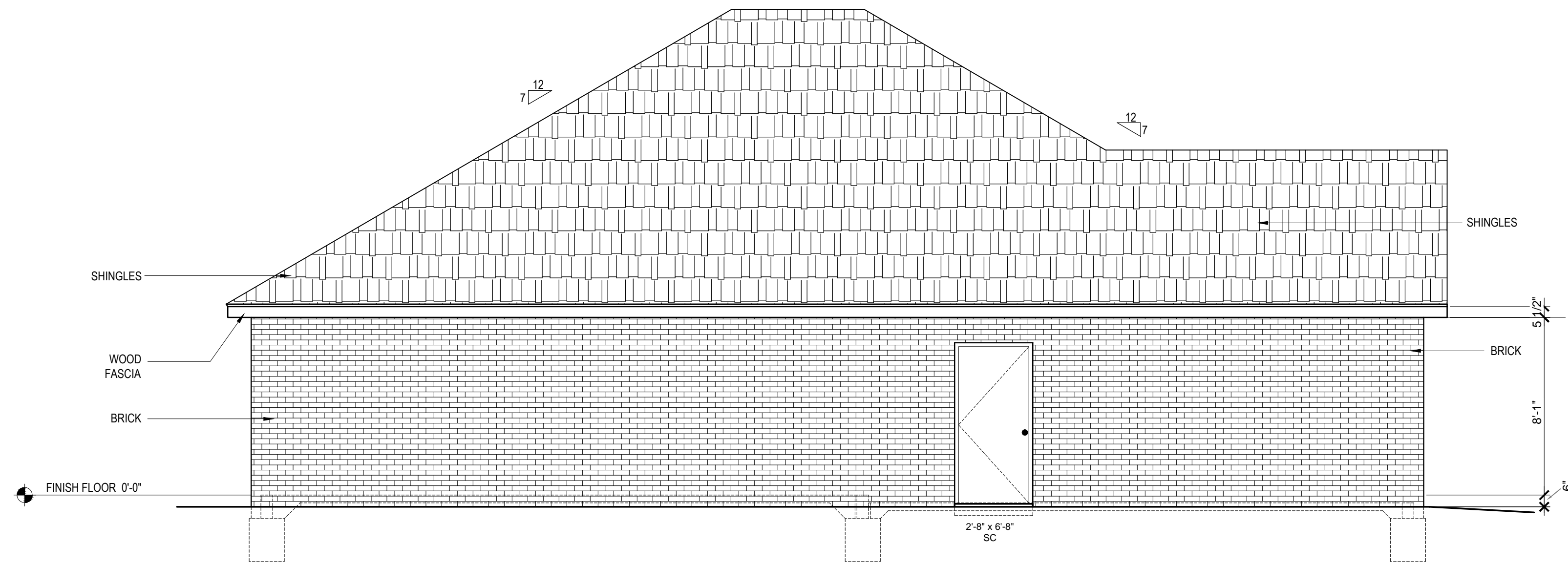
1 HOUSE 5M - SIDE ELEVATION SCALE: 1/4"=1'-0"
