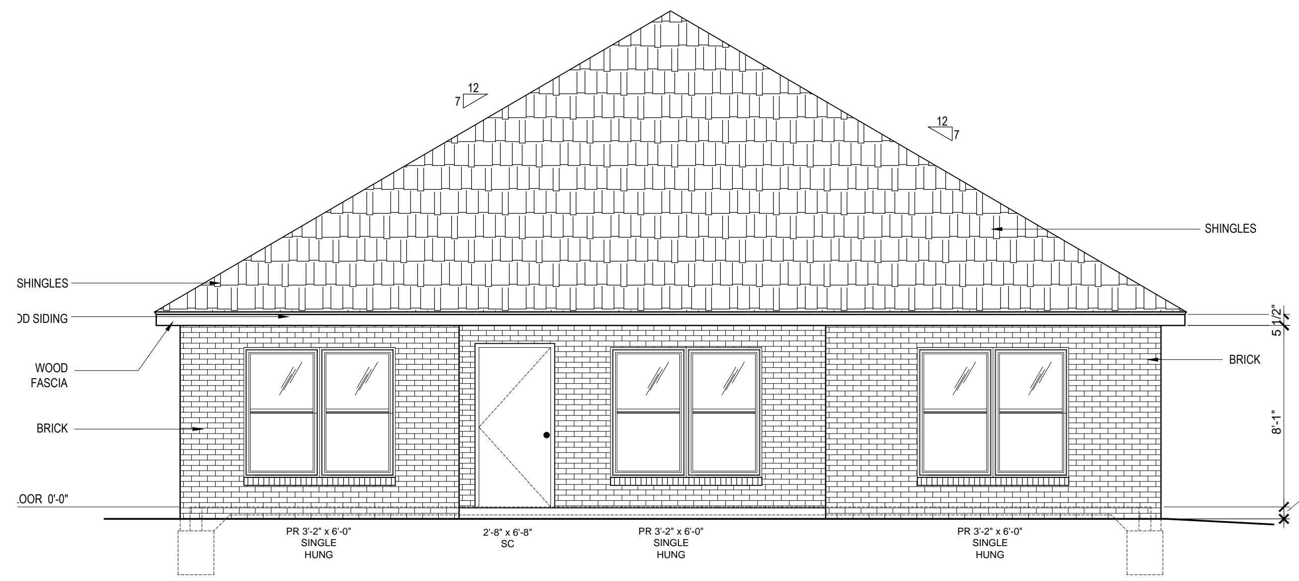
3 HOUSE 5M - REAR ELEVATION SCALE: 1/4"=1'-0"
