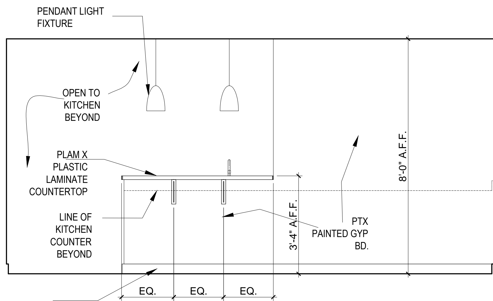
3 HOUSE 5M - PASS-THRU ELEVATION SCALE: 1/2"=1'-0"
