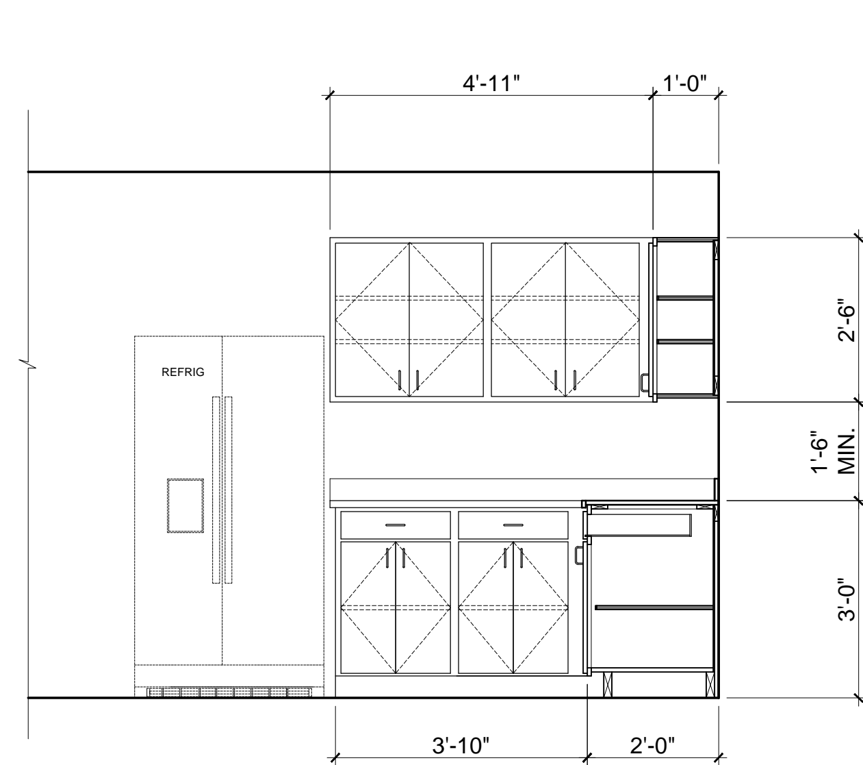
4 HOUSE 5M - KITCHEN ELEVATION SCALE: 1/2"=1'-0"
