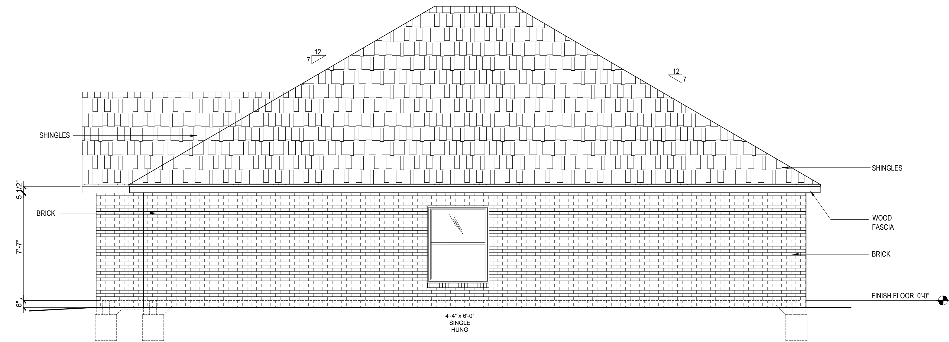
4 HOUSE 5M - SIDE ELEVATION SCALE: 1/4"=1'-0"
