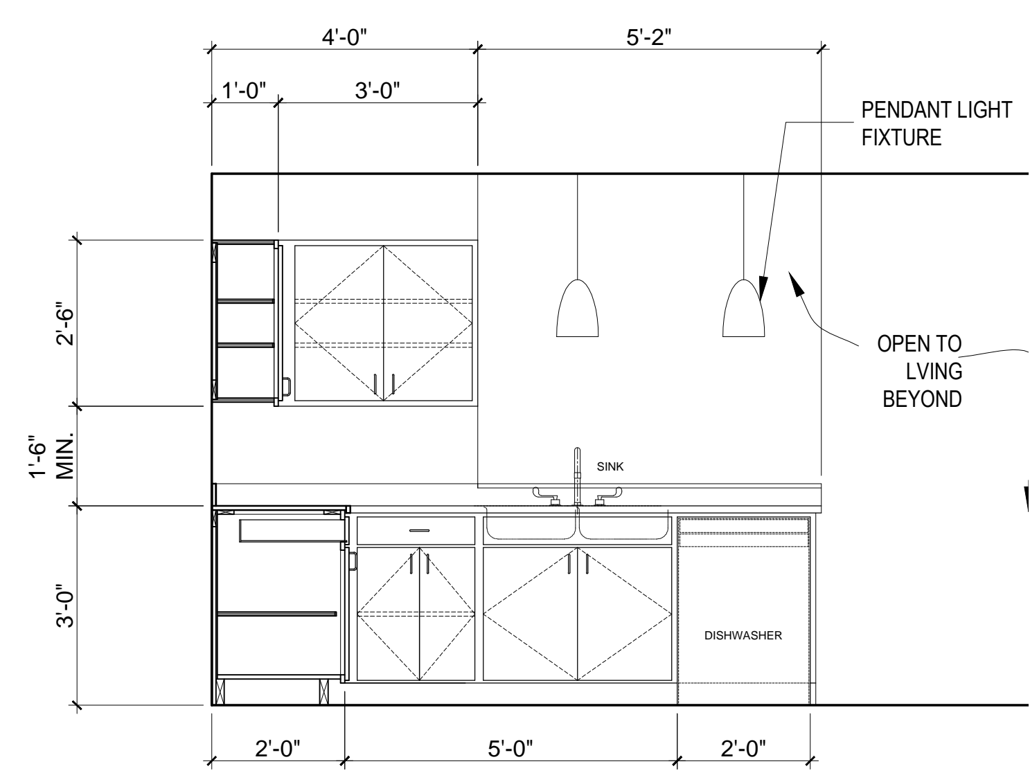
6 HOUSE 5M - KITCHEN ELEVATION SCALE: 1/2"=1'-0"
