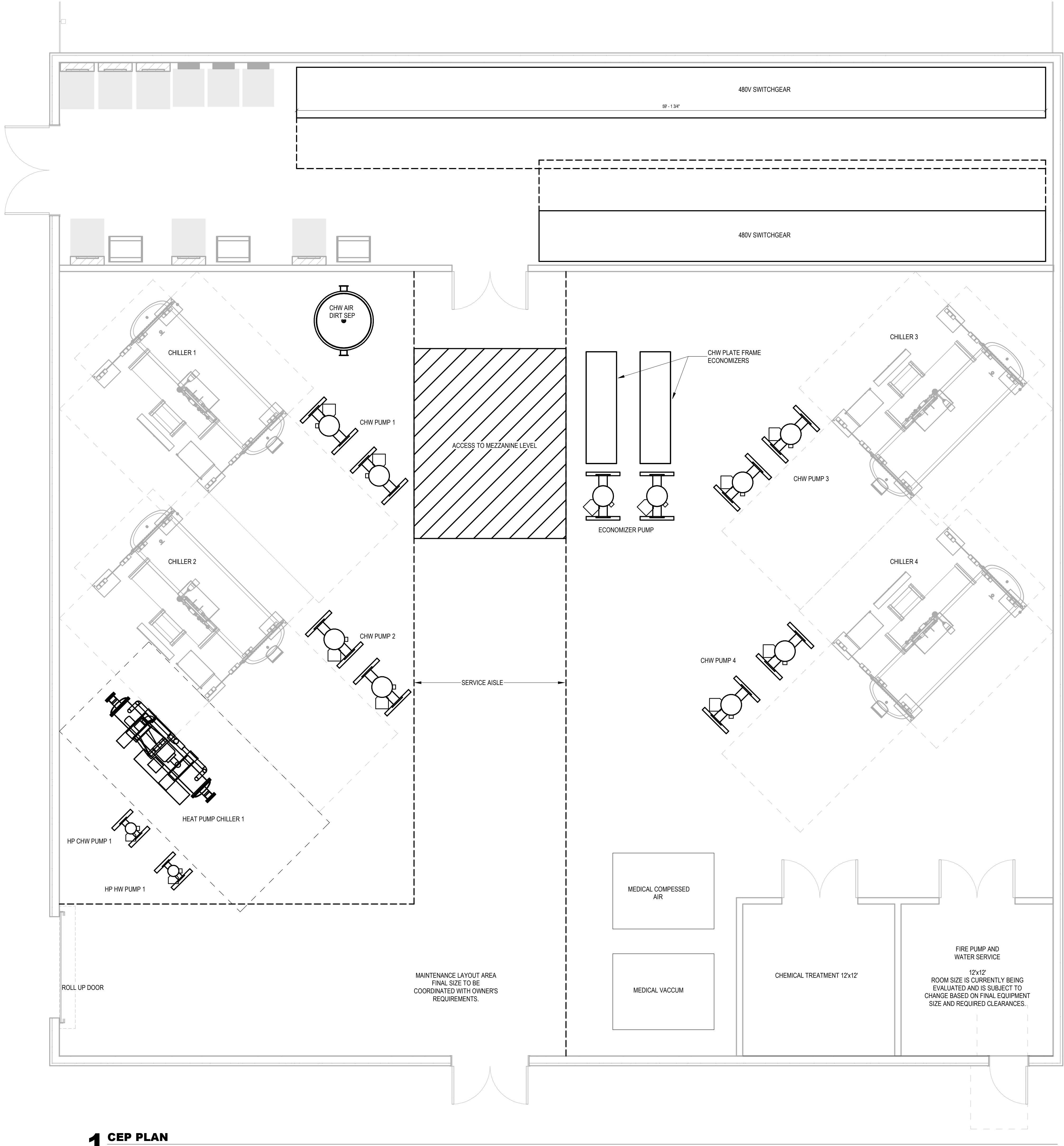
1 CEP PLAN 1/4" = 1'-0"
