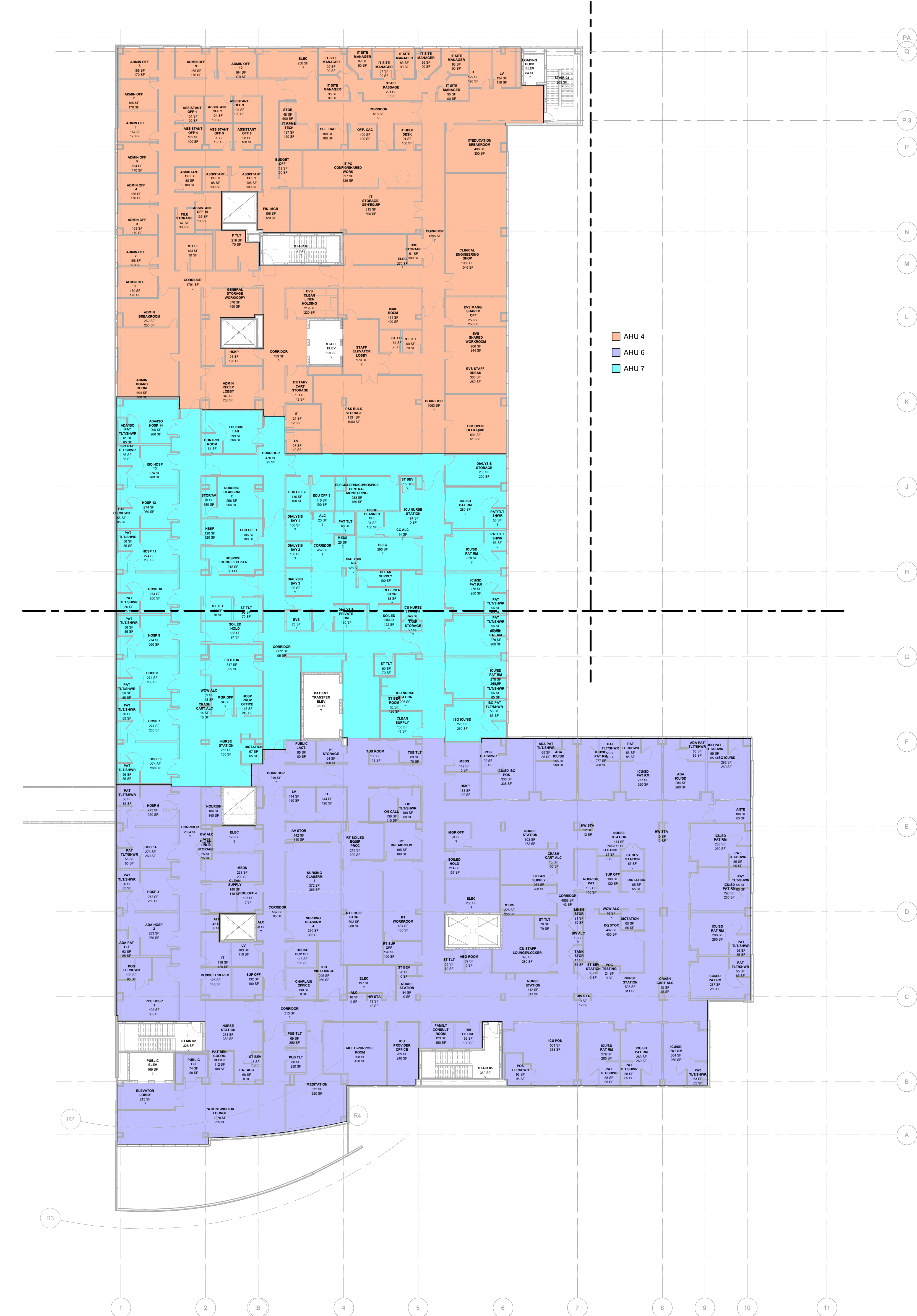
1 AHU ZONING - LEVEL 3 1" = 20'-0"
