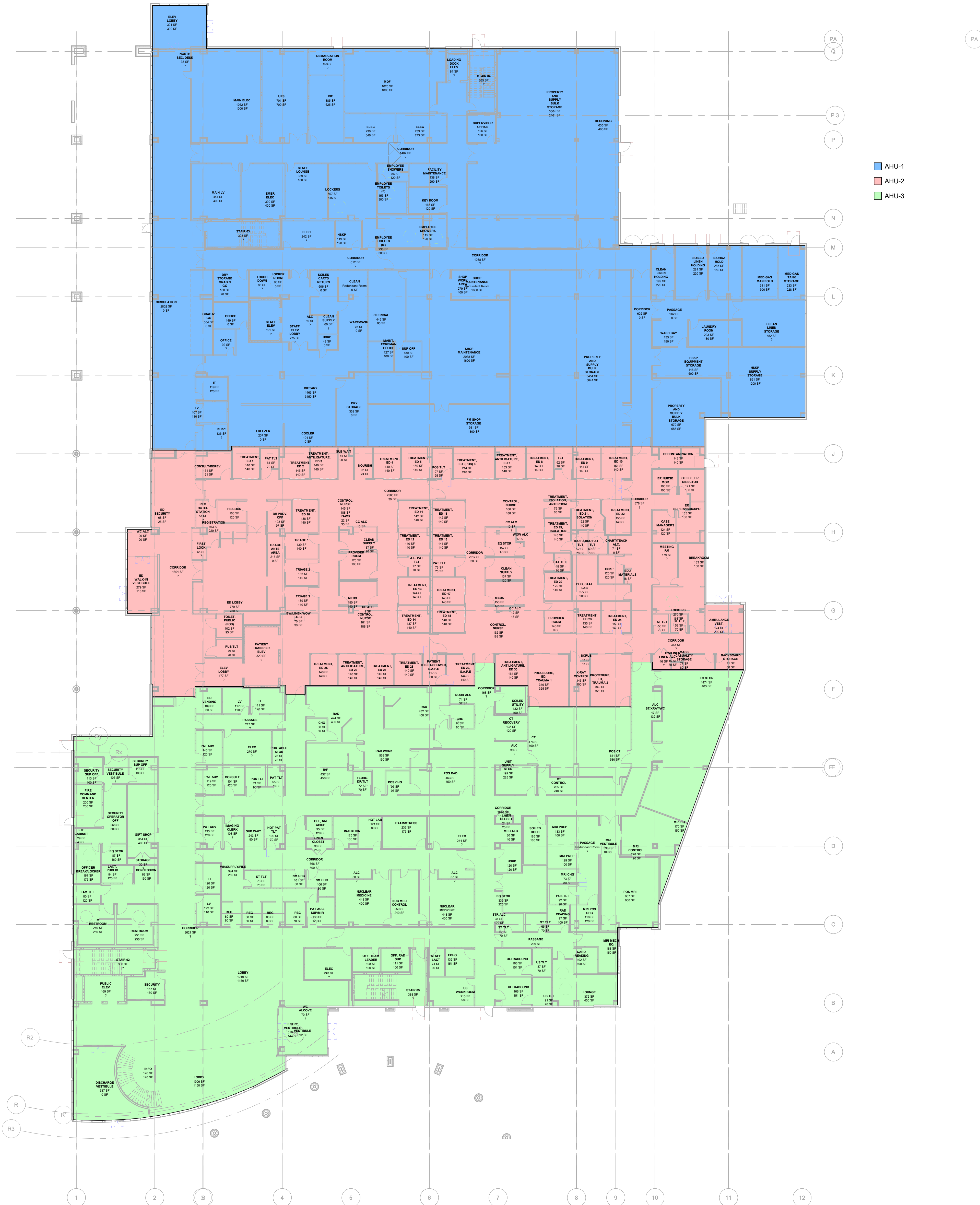
1 AHU ZONING - LEVEL 1 1" = 20'-0"
