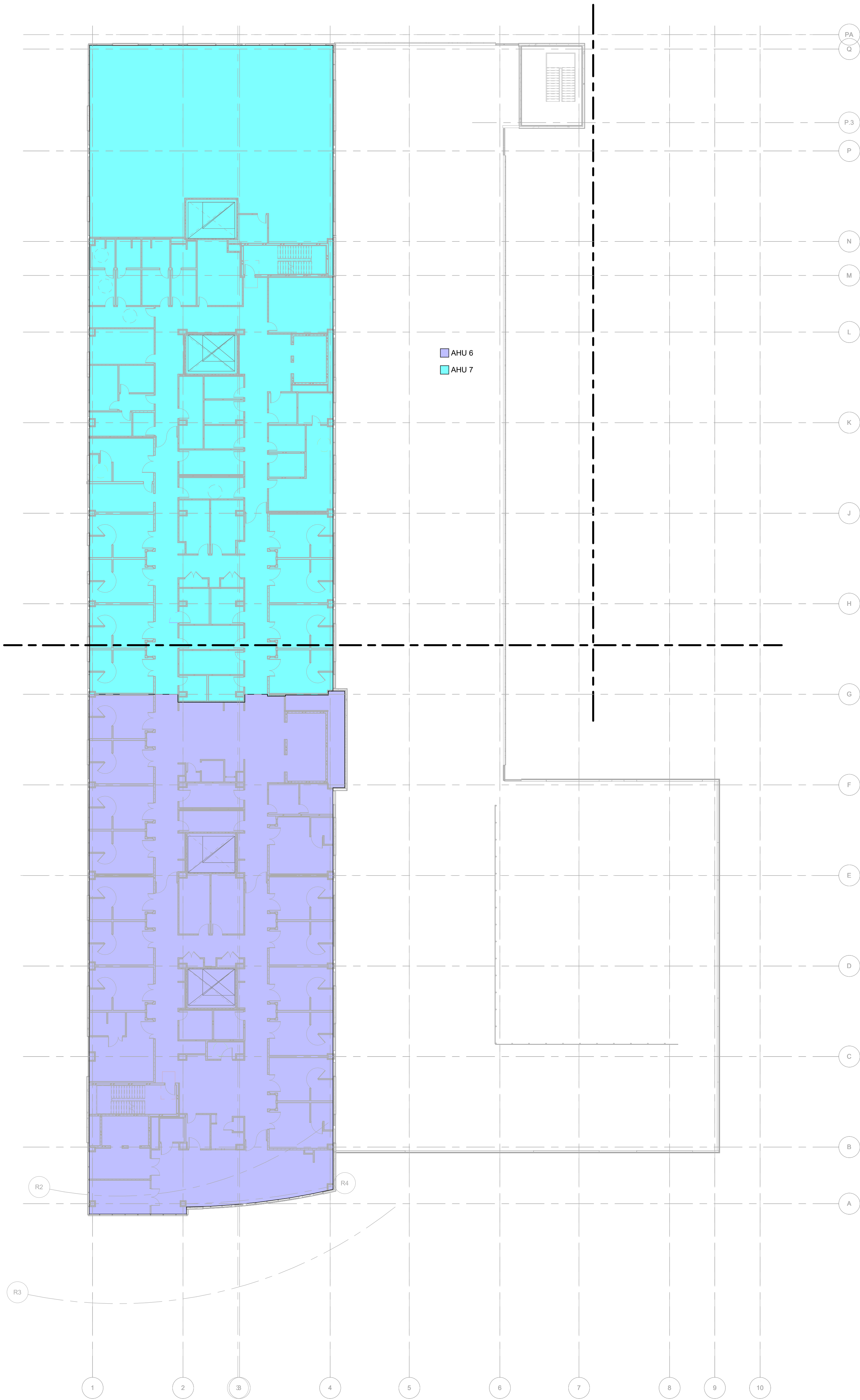
2 AHU ZONING - LEVEL 5 1" = 20'-0"
