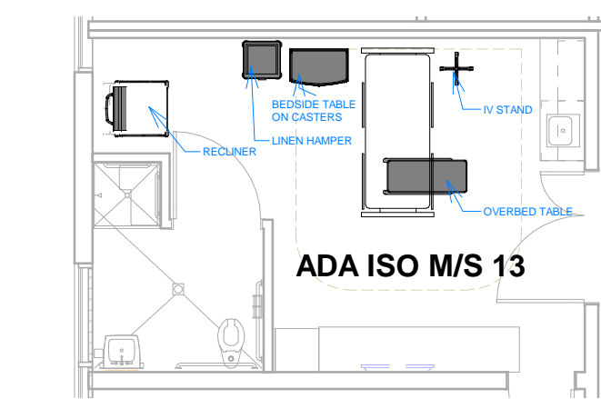
1 Level 06 - Acute Care - ISO M/S 1/8" = 1'-0"
