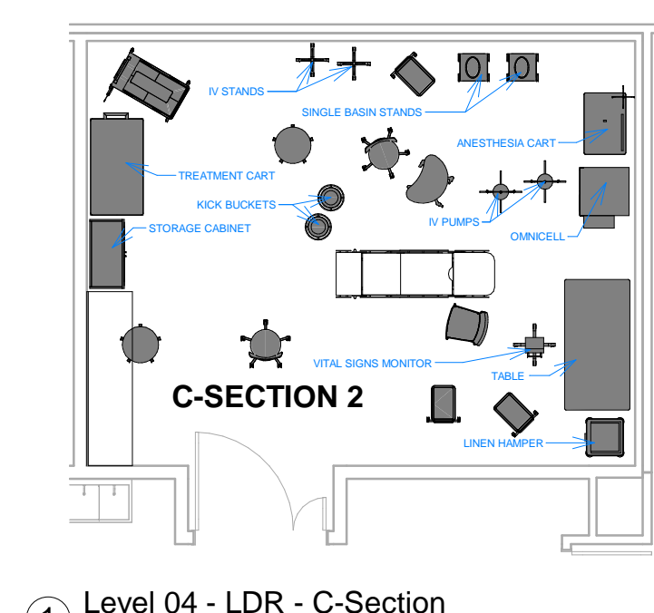
① Level 04 - LDR - C-Section 1/8" = 1'-0"
