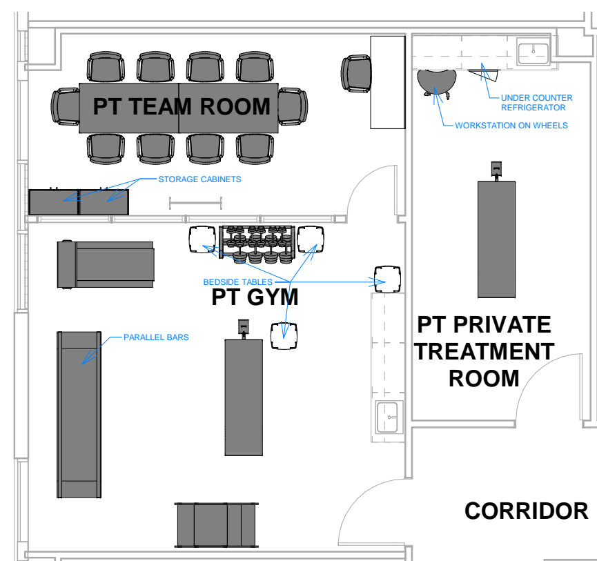
Level 06 - PT - Team Room/Gym/Private Treatment Room ③ 1/8" = 1'-0"
