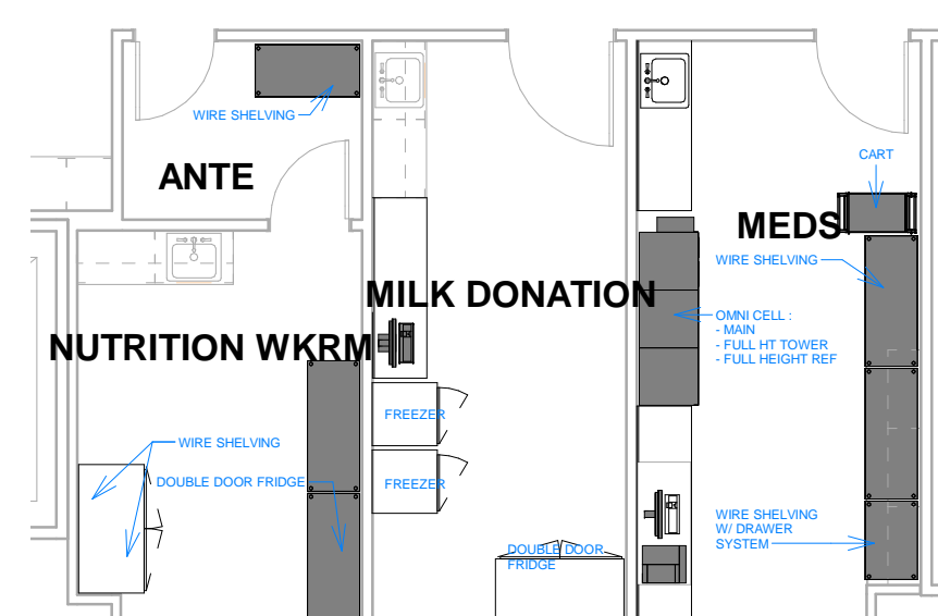
4 Level 04 - NICU - Ante/Nutrition Workroom/Milk Donation/Meds 1/8" = 1'-0"
