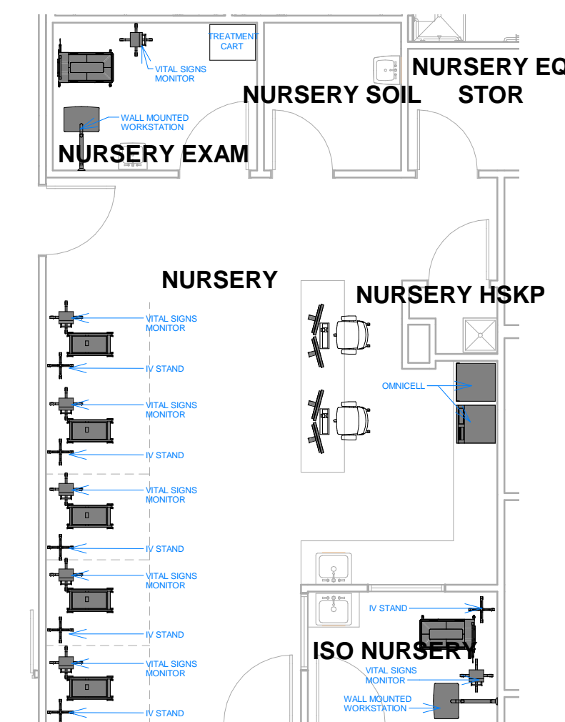
3 Level 04 - LDR - Nursery 1/8" = 1'-0"
