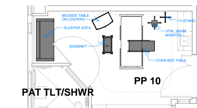
8 Level 04 - LDR - Post Partum 1/8" = 1'-0"
