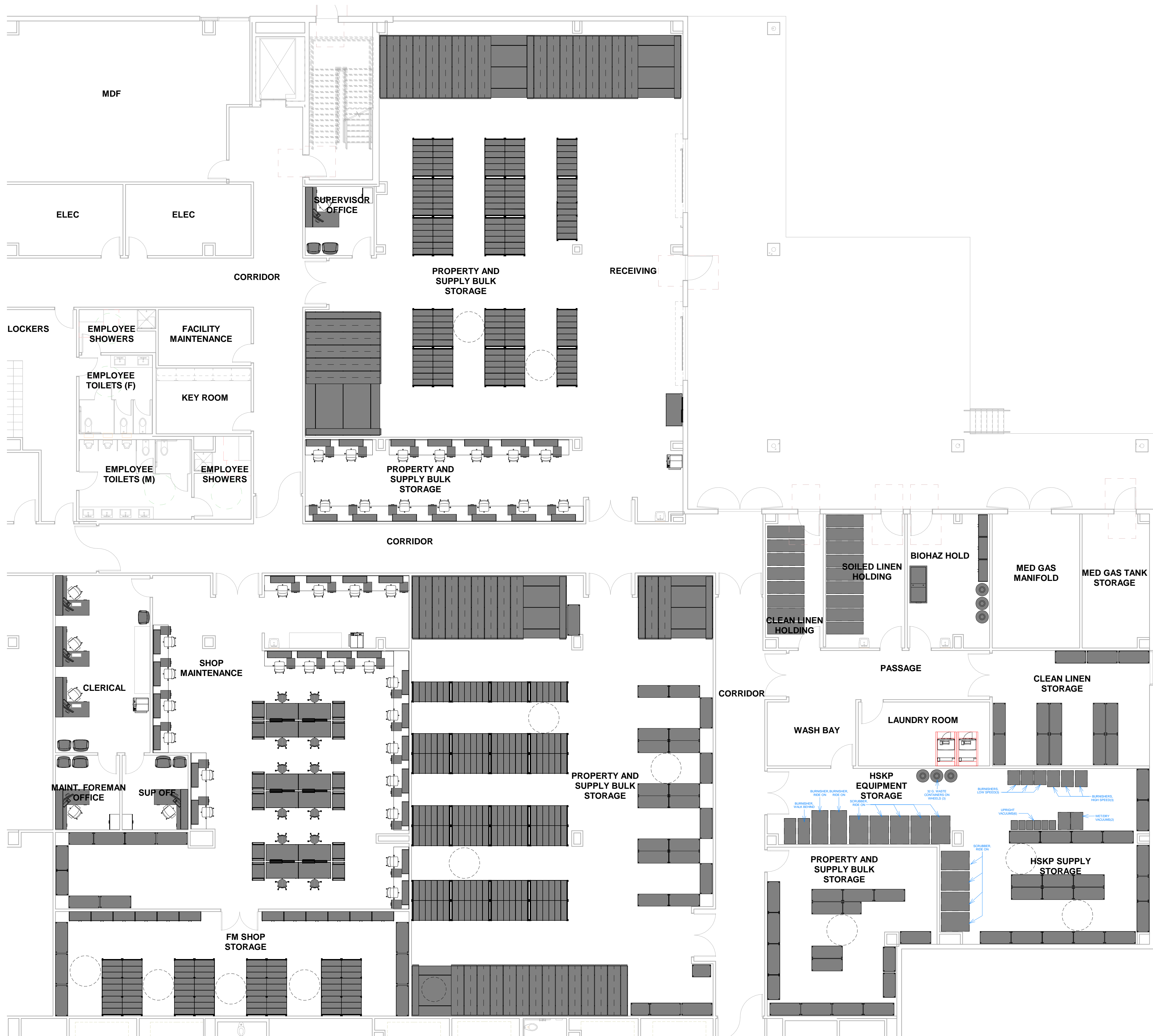
2 Level 01 - P&S/ Facilities Management/ Houskeeping & Linens 1/8" = 1'-0"
