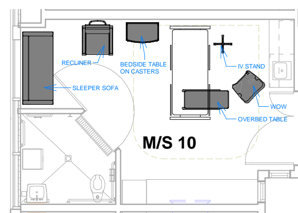
2 Level 06 - Acute Care - M/S Room 1/8" = 1'-0"
