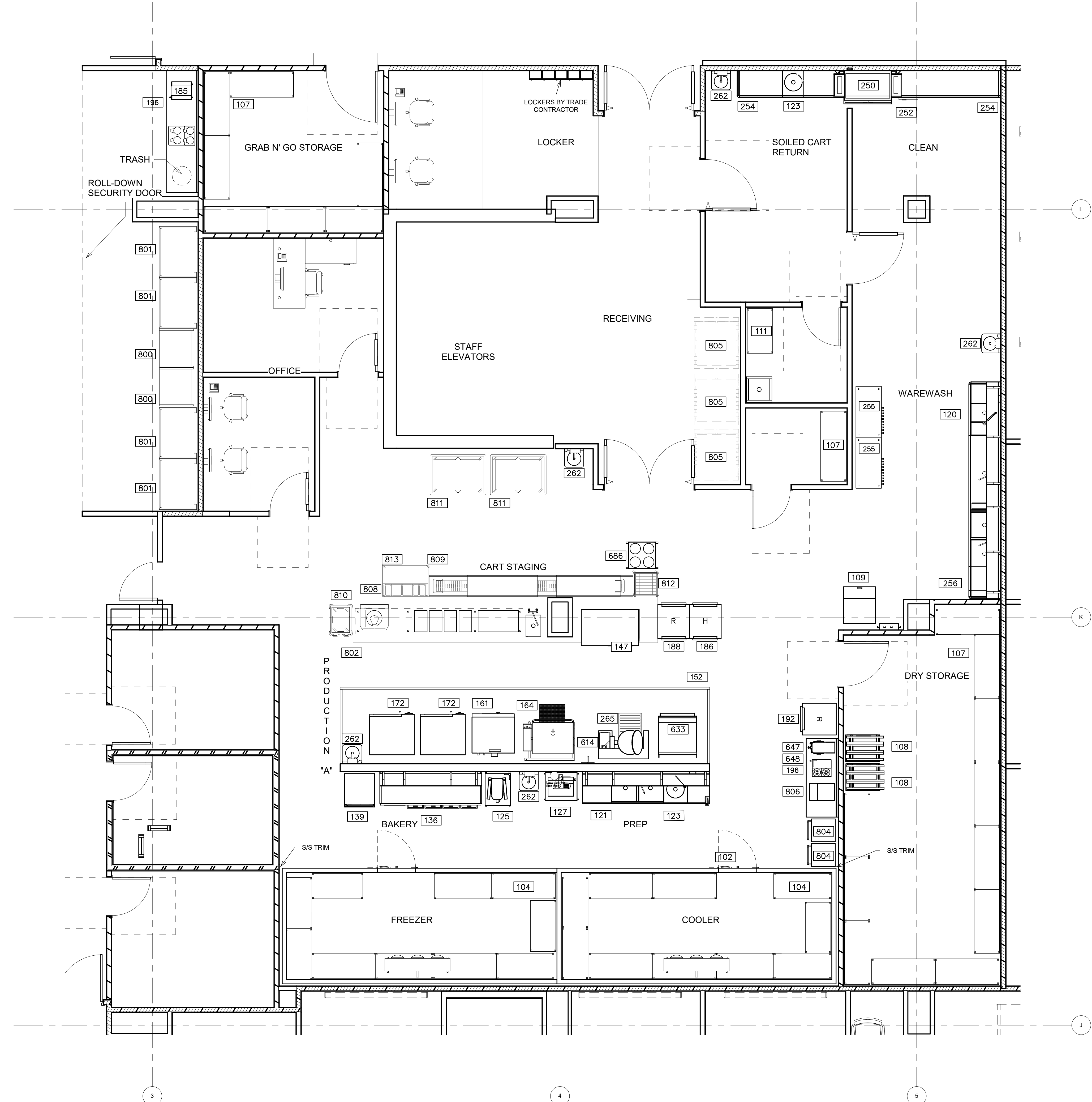
1 FOODSERVICE EQUIPMENT PLAN 1/4" = 1'-0"
