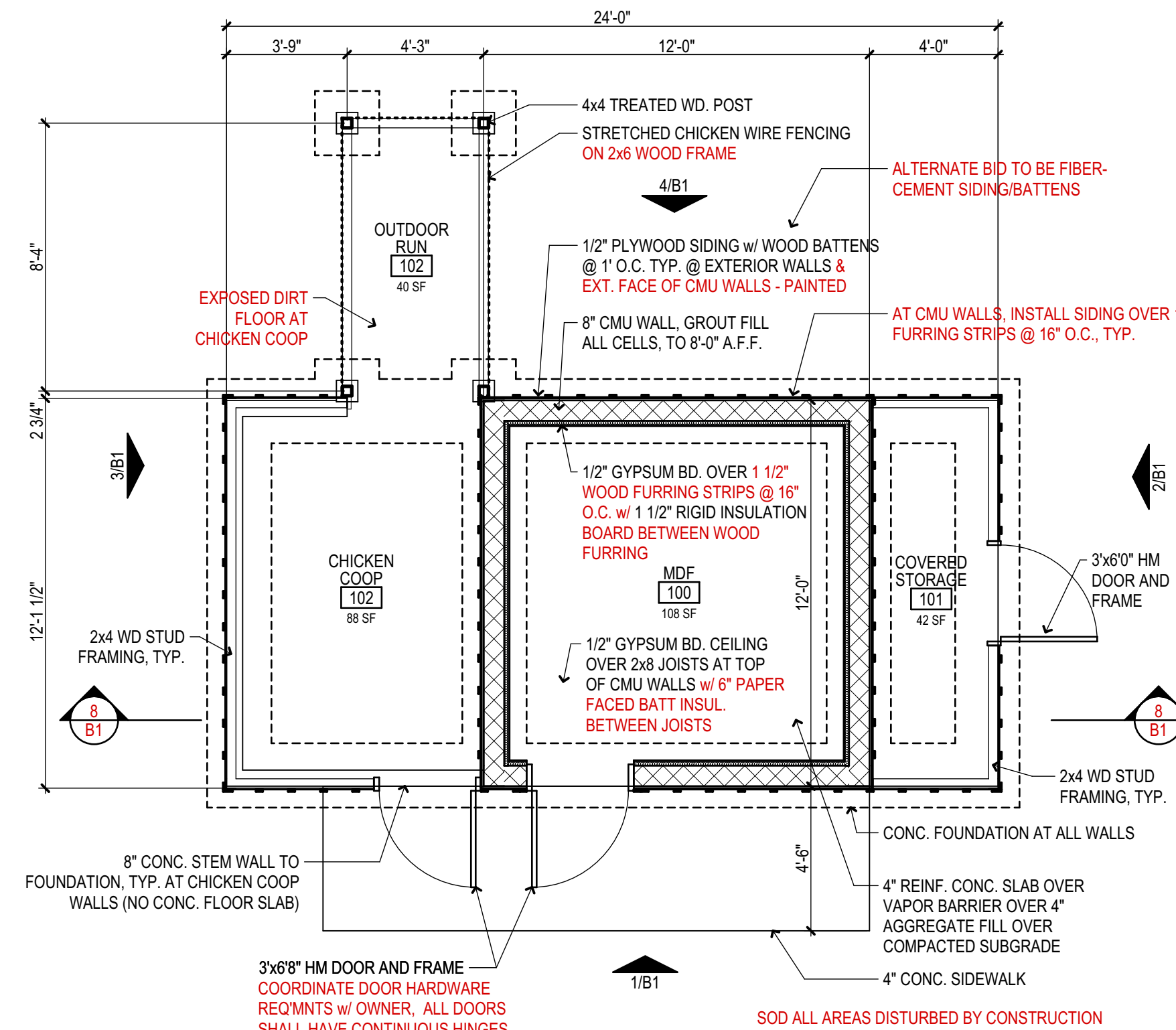
5 FLOOR PLAN
