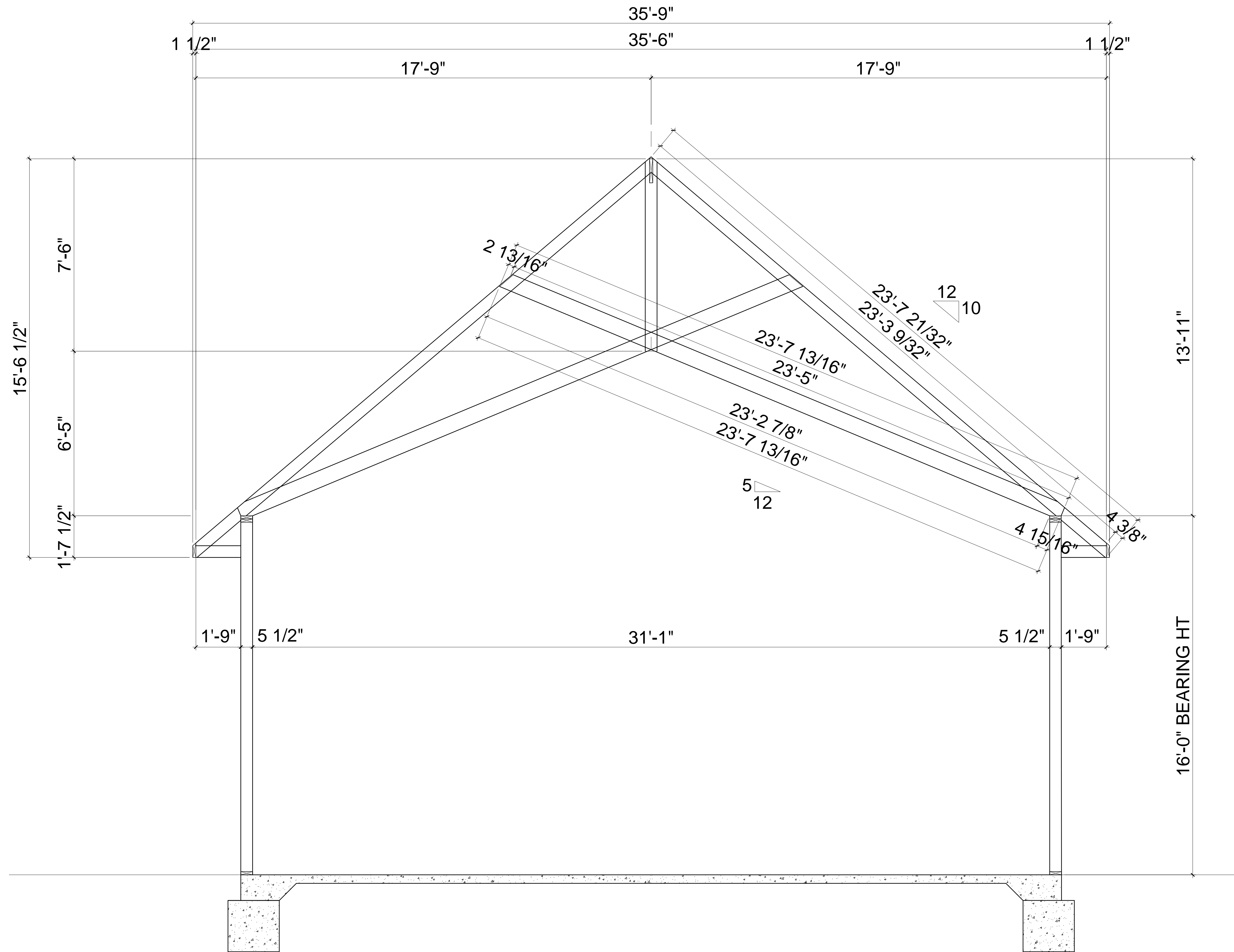
1 2 BED + LOFT SECTION THRU ROOF TRUSS SCALE: 1/2"=1'-0"
