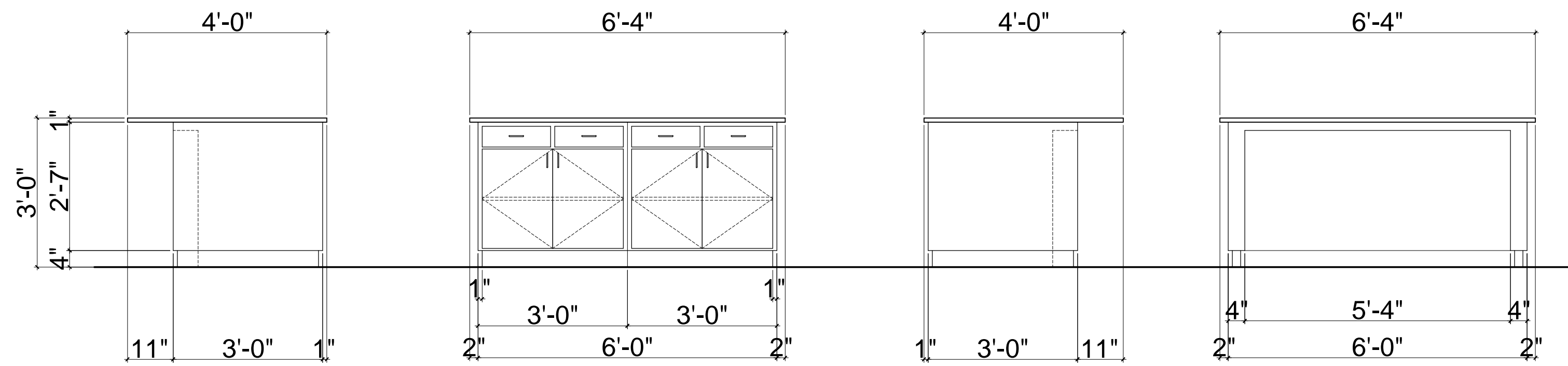
5 3 BED + LOFT CABIN - KITCHEN ISLAND ELEVATIONS SCALE: 1/2"=1'-0"
