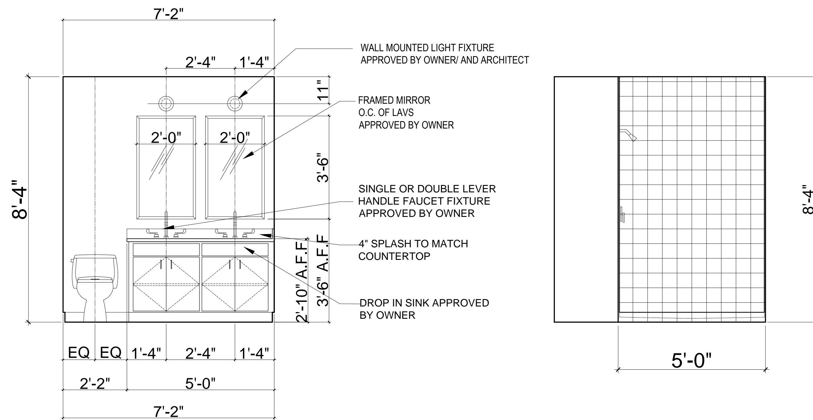
3 3 BED + LOFT CABIN - TOILET ELEVATION SCALE: 1/2"=1'-0"
