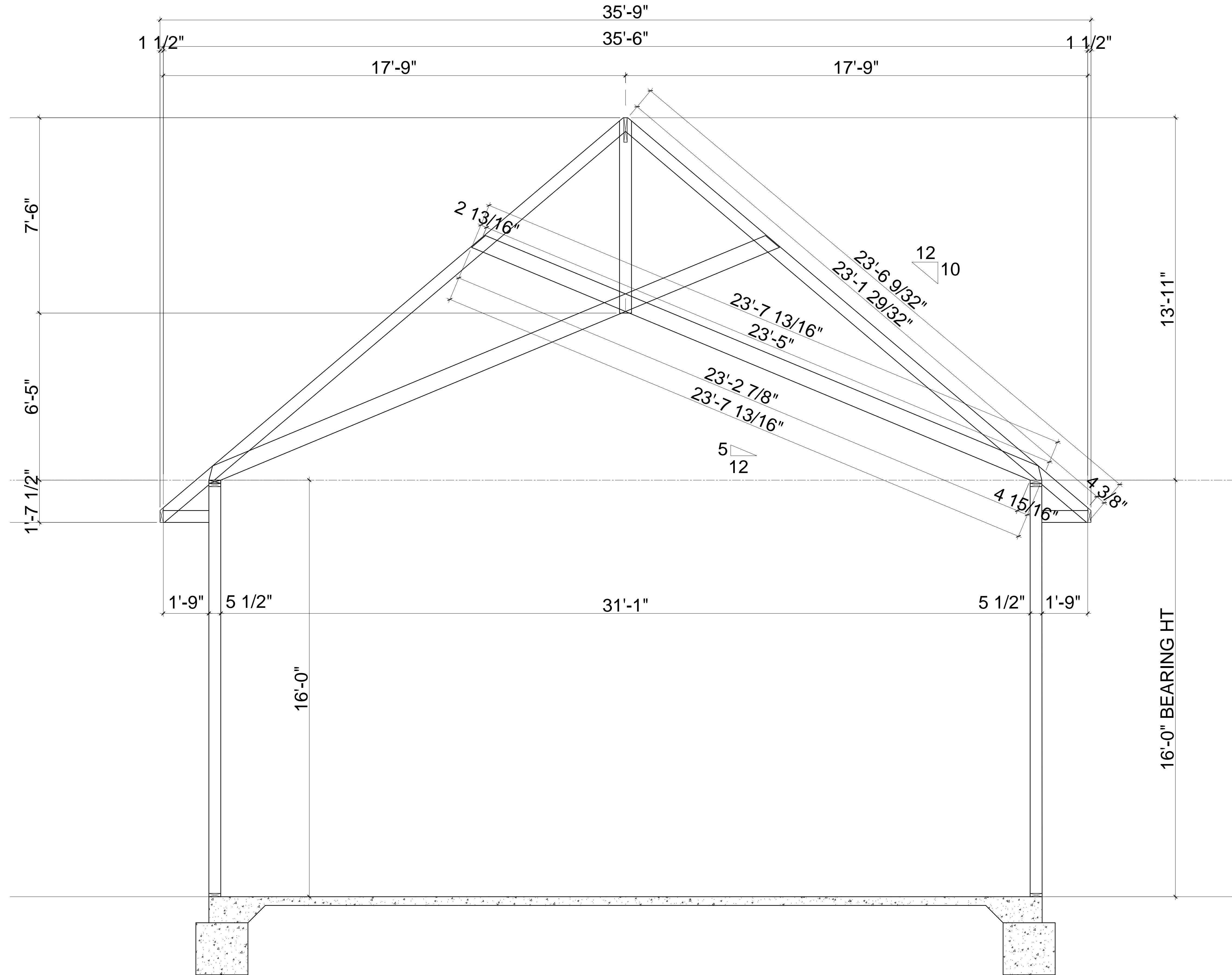
3 4 BED + LOFT SECTION THRU ROOF TRUSS SCALE: 1/2"=1'-0"
