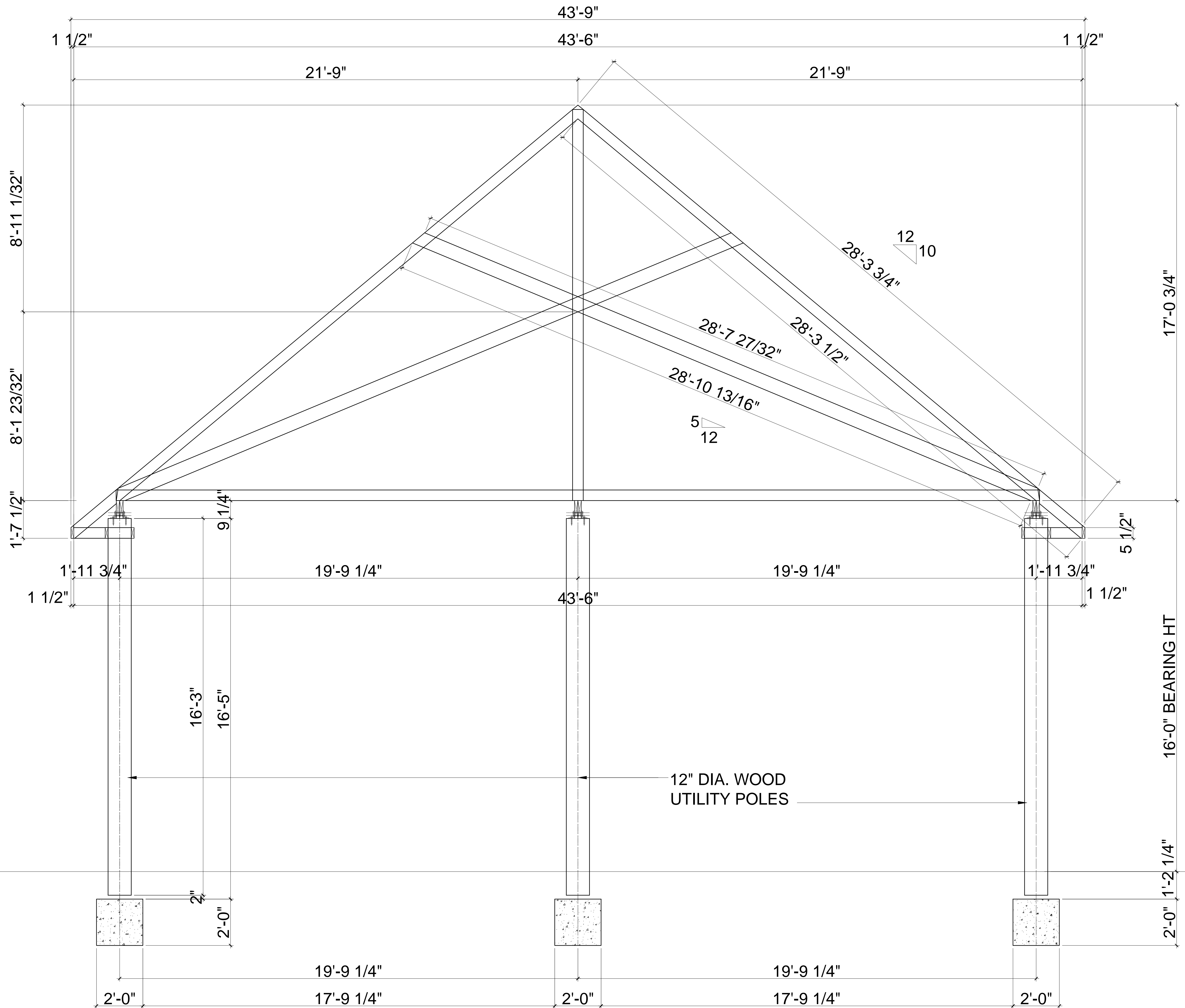
1 6 BED + LOFT - GABLE END ROOF TRUSS SCALE: 1/4"=1'-0"
